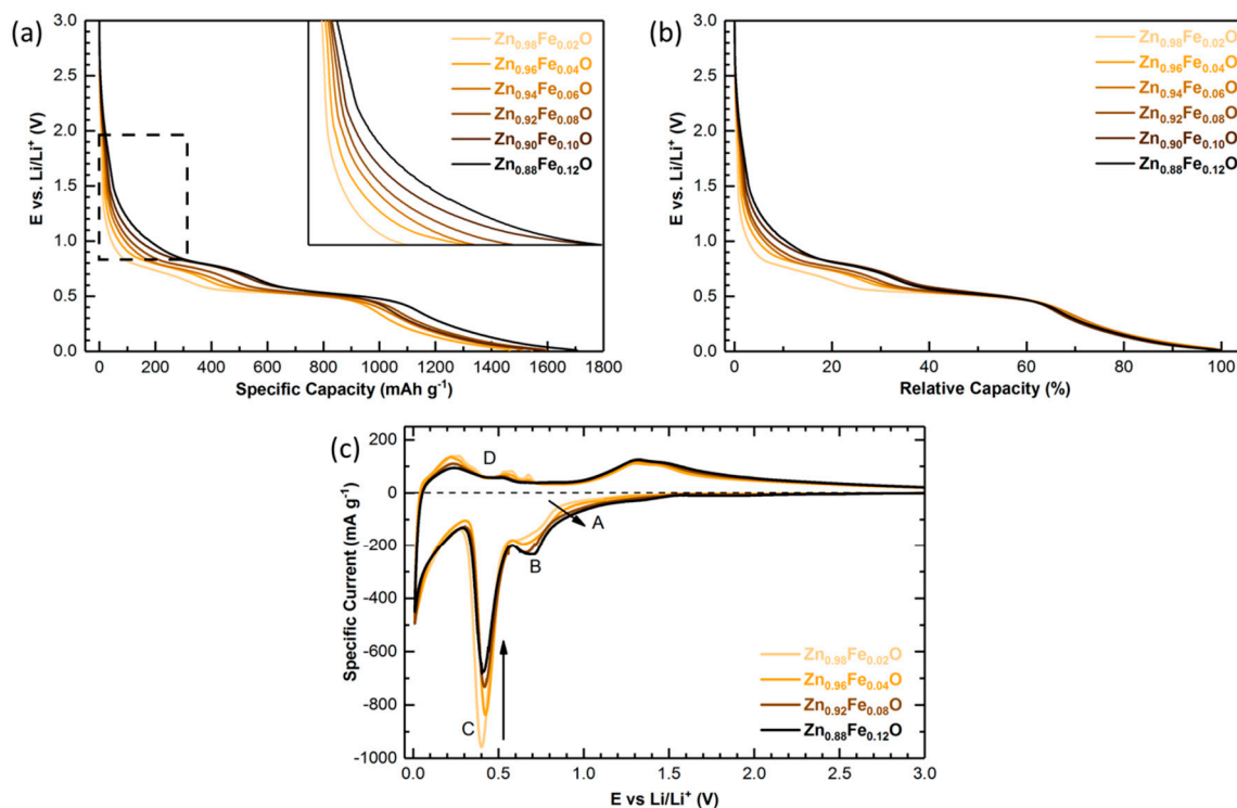
Figure 6. (a) Potential profiles for the first galvanostatic discharge of \text{Zn}_{1-x}\text{Fe}_x\text{O} -based electrodes ( x = 0.02, 0.04, 0.06, 0.08, 0.10, and 0.12 ), applying a discharge rate of 0.05\text{C} (i.e., 48.3 \text{ mA g}^{-1} ); the inset shows a magnification of the area highlighted by the dashed box; (b) The same potential profiles as presented in (a), but plotted versus the normalized capacity; (c) Cyclic voltammetry conducted for selected samples ( x = 0.02, 0.04, 0.08, and 0.12 ), applying a sweeping rate of 50 \mu\text{V s}^{-1} .
