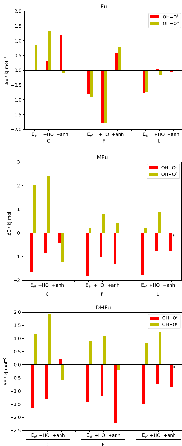
FIG. 7. Computed relative energies for three submissions from electronic energy ( E_{el} ), adding harmonic ZPVE corrections (+HO) and adding anharmonic correction terms. Further details are provided in the text. All values are shown relative to the OH- \pi dimer.
