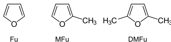
FIG. 1. Lewis structures of the furans featured in the study and the abbreviations used throughout the text: furan (Fu), 2-methylfuran (MFu) and 2,5-dimethylfuran (DMFu).
