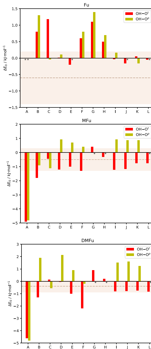
FIG. 6. Computed relative internal energies (0 K) for each submission (labels explained in Table II). All energies are shown relative to the OH- \pi dimer. The asterisks denote missing values. The dashed line plus shaded section represent the experimentally derived value and respective error bounds.
