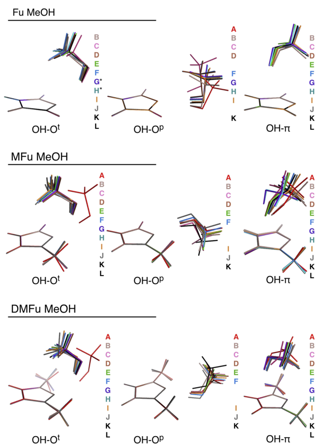
FIG. 4. Overlap of selected structures from the submissions, grouped according to the binding motif. To the right of the structures is a list of the entries which included the motif. The asterisk denotes transition state structures.
