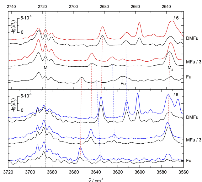
FIG. 3. Spectra of the mixtures of the three different furans with methanol. Spectra with pure MeOH in blue, with pure MeOD in red, and MeOH/MeOD mixtures in black. The spectral regions of OH and OD stretching vibrations are stacked so that MeOH ( 3686\text{ cm}^{-1} ) and MeOD monomer ( 2718\text{ cm}^{-1} ) are aligned and the OD region is scaled by \sqrt{2} .
