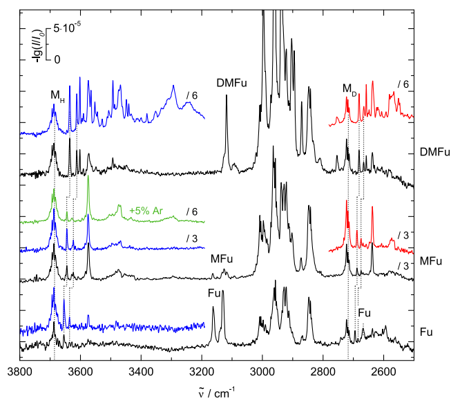
FIG. 2. Spectra of the mixtures of the three different furans with methanol. Spectra with pure MeOH in blue, with pure MeOD in red, and mixtures in black. The green trace for MFu shows the effect of adding 5% Ar to the expansion (see text).
