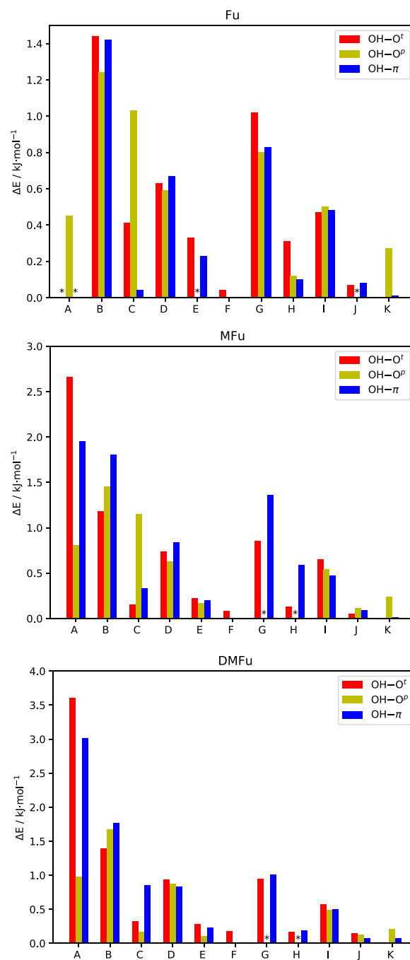
FIG. 5. Relative electronic energies (in kJ/mol) computed for each geometry of a specific conformer. All values are plotted relative to the lowest lying value found among all sets for each distinct conformer. The single point energies were computed at the CCSD(T)-F12/cc-pVTZ-F12 level of theory. The asterisks denote missing structures.
