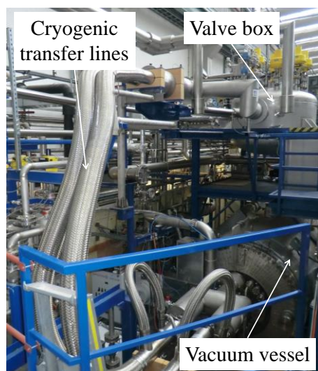
Figure 2. TIMO-2 facility.
