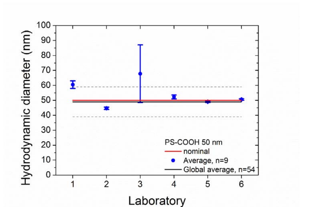
Figure 6b. Results from the third ILC round by DCS. Mass-based hydrodynamic modal diameter results for 50 nm PS-COOH NPs dispersed in water. Dashed lines correspond to \pm 2 \times ILC SD; error bars correspond to \pm 1 \times lab SD.
