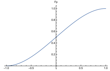
Figure 2. cdf of (7) in the case p = 5
