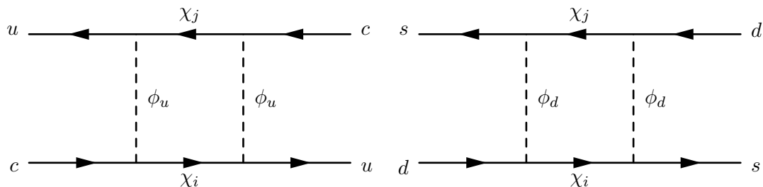
Figure 3. New one loop contribution to D^0 - \bar{D}^0 (left) and K^0 - \bar{K}^0 mixing (right). Analogous contributions to B_d^0 - \bar{B}_d^0 and B_s^0 - \bar{B}_s^0 mixings exist.
