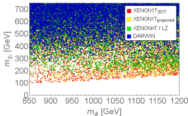
Figure 8. Viable area in the m_\phi - m_{\chi_t} plane of the quark doublet DMFV model with combined flavour, relic abundance and direct detection constraints applied in the QDF scenario, for \eta = -0.01 . We show the viable ranges for different strengths of direct detection bounds. The current exclusion bounds of XENON1T [43] as well as the projected bounds of XENON1T [45], XENONnT [45], LUX-ZEPLIN (LZ) [46] and DARWIN [47] are applied respectively. The interference of relic abundance and direct detection effects results in a lower bound on the DM mass, increasing with more stringent direct detection bounds.
