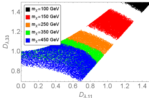
Figure 5. Viable regions of parameter space of the quark-doublet DMFV model in the QDF scenario (with m_{\phi} = 850 GeV and \eta = -0.01 ) compatible with the relic abundance constraint, at different DM masses.
