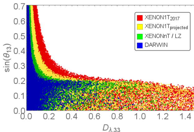
Figure 6. Viable areas of parameter space of the quark doublet DMFV model, for different WIMP nucleon scattering cross section limits, for DM mass m_\chi = 250 GeV and mediator mass m_\phi = 850 GeV. The current exclusion bounds of XENON1T [43], as well as the projected bounds of XENON1T [45], XENONnT [45], LUX-ZEPLIN (LZ) [46] and DARWIN [47] have been imposed respectively. Note that in this scan we did not impose any of the other constraints discussed before, as we focus on the bare influence of the direct detection bounds.
