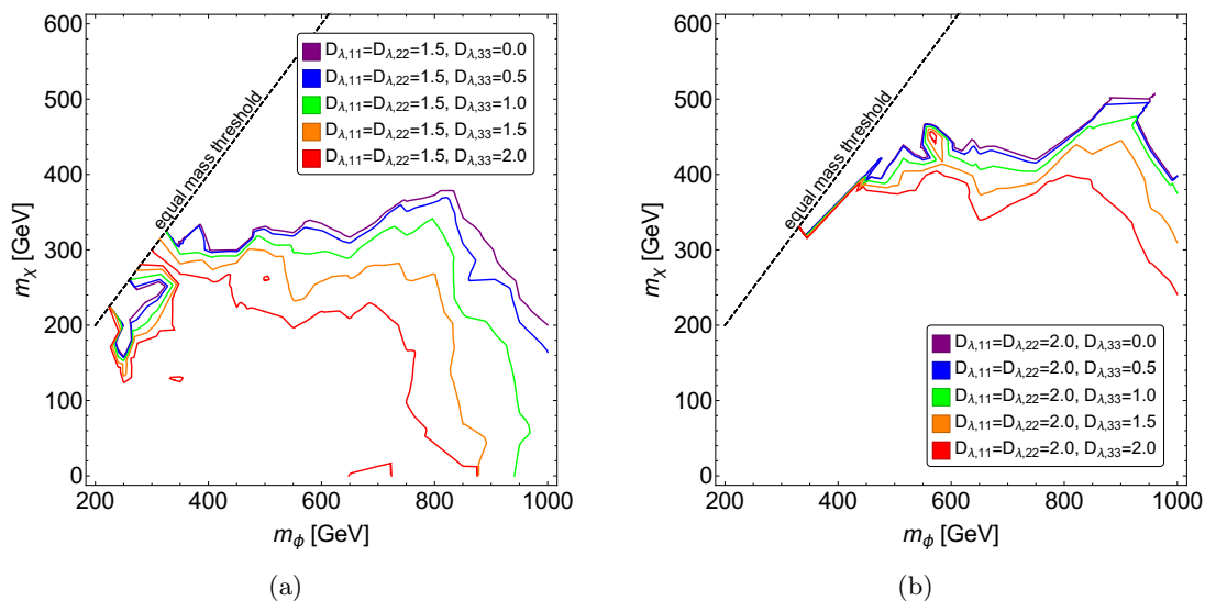
Figure 2. Constraints on the jets + \cancel{E}_T final state from 8 TeV LHC run 1 data, obtained from the cross-section limits in [31]. Left: 95% C.L. exclusion contours of the quark-doublet DMFV model for various strengths of third generation couplings, with fixed D_{\lambda,11} = D_{\lambda,22} = 1.5 . Right: 95% C.L. exclusion contours of the quark-doublet DMFV model for various strengths of third generation couplings, with fixed D_{\lambda,11} = D_{\lambda,22} = 2.0 , and the mixing angles \theta_{ij} set to zero. Note that, as discussed in detail in [22], the latter do not affect the identified safe parameter space.
