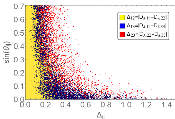
Figure 4. Viable ranges for the flavour mixing angles \theta_{ij} of the quark doublet DMFV model in dependence of the splittings between couplings D_{\lambda,ii} and D_{\lambda,jj} , for mediator mass m_\phi = 850 GeV and DM mass m_\chi = 250 GeV. Different colours correspond to the different mixing angles \theta_{ij} and splittings |D_{\lambda,ii} - D_{\lambda,jj}| = \Delta_{ij} , with each colour representing one pair of indices: ij = 12 in yellow, ij = 13 in blue, ij = 23 in red.
