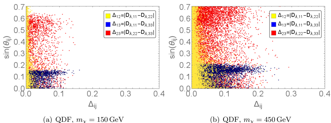
Figure 7. Viable regions of parameter space of the quark doublet DMFV model, with combined flavour, relic abundance and direct detection constraints applied, for QDF scenario and different DM masses, with m_\phi = 850 GeV and \eta = -0.01 . Different colours correspond to the different mixing angles \theta_{ij} and splittings |D_{\lambda,ii} - D_{\lambda,jj}| = \Delta_{ij} , with each colour representing one pair of indices: ij = 12 in yellow, ij = 13 in blue, ij = 23 in red.
