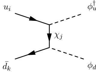
Figure 1. Relevant production channel for \phi_u\phi_d mixed state.
