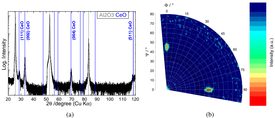
Fig. 4.12: XRD characterization of the CeO 2 buffer layer. (a) \theta - 2\theta scan of a 20 nm CeO 2 film on sapphire substrate. (b) texture of the (103) plane of a YBCO film grown on a CeO 2 buffer.
