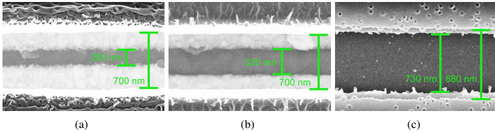
Fig. 5.4: SEM images of slit dimensions etched with (a) IBE, (b) oxygen-plasma assisted IBE and (c) the I_2(KI)_5 solution in 1:3 dilution. The green markers indicate the width of the etched gold slit and of the resist mask, respectively. During wet-chemical etching the resist mask is underetched (see (c)). As the PMMA resist is not stable under electron bombardment, it melts during SEM imaging.
