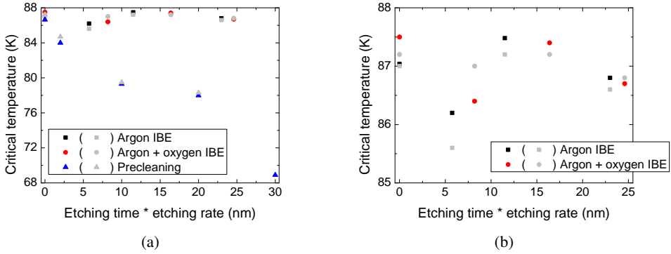
Fig. 5.3: Influence of argon-ion bombardment on the critical temperature for samples processed with the three different systems. The measured values of the critical temperature directly after treatment and after one month of storing in a desiccator are displayed as a function of the over-etching. The over-etching is displayed as the equivalent gold thickness that would be etched during the etching time (etching rate * etching time). Over-etching of up to 25 nm of gold was tested. (a) Comparison of all three etching techniques, (b) detailed view of the results achieved with the IBE system with pure argon-ion milling and with oxygen-assisted argon-ion milling.
