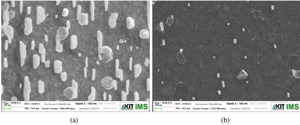
Fig. 4.16: SEM pictures of interval-deposited PBCO: (a) n_p = 14 pulses per ML, (b) n_p = 15 pulses per ML [FeB16]. The layer thickness is four MLs.
