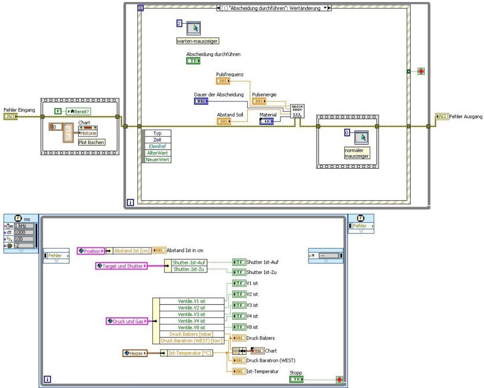
Fig. 4.4: LabVIEW block diagram. The laser ablation step within the semi-automated process is shown.
