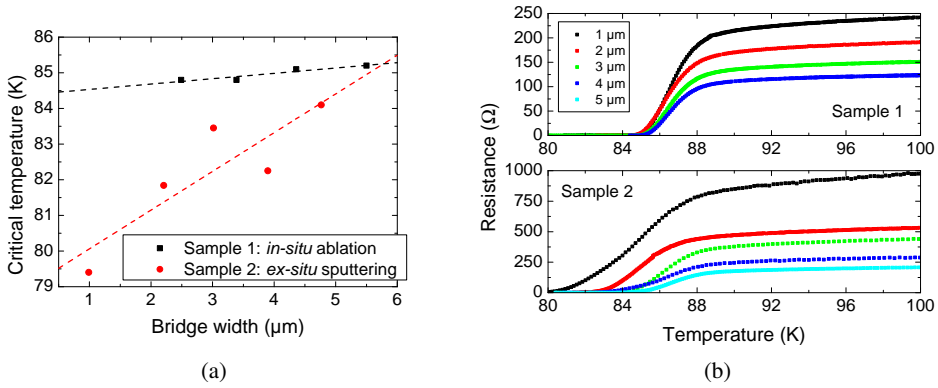
Fig. 4.19: (a) Dependence of the critical temperature on the bridge width for in-situ ablated and ex-situ sputtered gold films deposited on top of a \text{CeO}_2/\text{PBCO}/\text{YBCO}/\text{PBCO} multi stack, with lines to guide the eye, and (b) corresponding R(T) curves.
