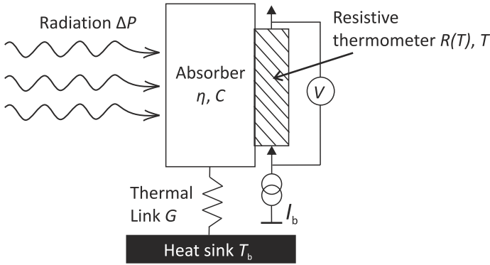
Fig. 2.7: Operation principle of a bolometric detector in composite design with current bias, adapted from [48].
