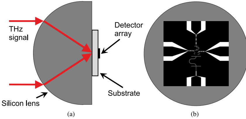
Fig. 6.6: Off-centered antenna elements in the four-pixel detector array: (a) side view of the hyper-hemispherical silicon lens with the sapphire substrate glued to the flat side and (b) front view with the detector array placed on the silicon lens. The individual antennas are off-centered. The size of the array and the lens are not to scale.
