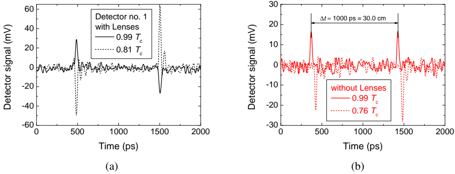
Fig. 6.19: Signal traces recorded with the Gouy phase-shift setup: (a) two traces with the Gouy phase shift at different temperatures measured with detector no. 1. The polarity of the recorded pulses is reversed. (b) Same measurement without the lenses, thus without a phase shift on the upper optical path in Fig. 6.18. No reversal of the pulse polarity is observed.
