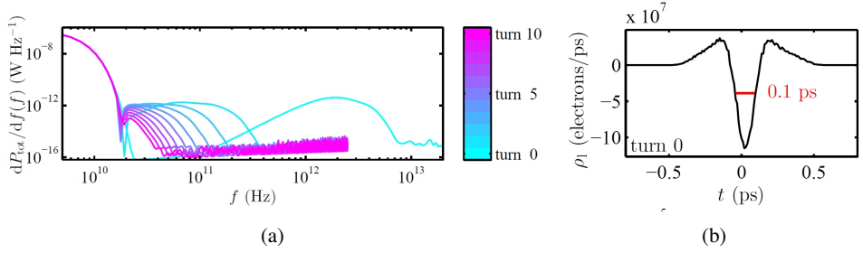
Fig. 2.4: (a) Spectral power density of the emitted THz signal from Coherent Harmonic Generation (CHG) for the first 11 revolutions of the bunch inside the synchrotron [27, p. 57]. The maximum at low frequencies corresponds to the coherent emission of the overall bunch length, which is not transmitted through the beamline. (b) Electron density modulation on the bunch for "turn 0" [27, p. 55].
