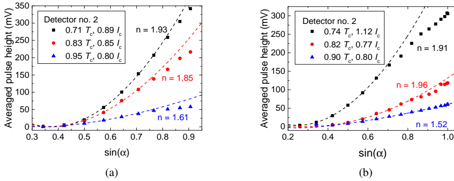
Fig. 7.5: Dependence of the detector response on coupled electrical field strength ( \sin(\alpha) ) and temperature for detector no. 2 (a) at 1.3 THz at FELBE and (b) at the IR2 beamline at ANKA. The dashed lines correspond to power-law fits as in Fig. 7.1(a) ( |U_{\max}| \propto \sin^n(\alpha) ). The exponents n of the interpolated data sets are given in the plots.
