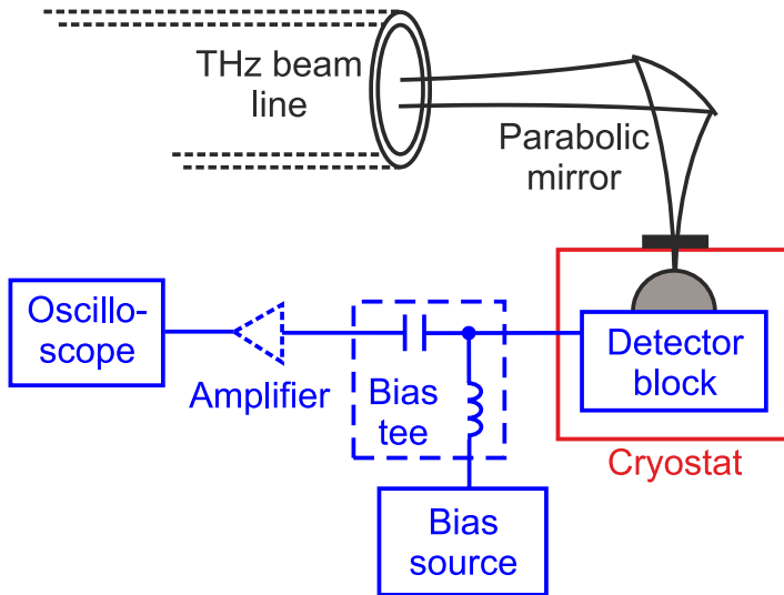
Fig. 6.1: Schematic of the YBCO detection system for pulsed THz excitations consisting of a cryostat (red) and the electronics (blue). The optical path is depicted in black.
