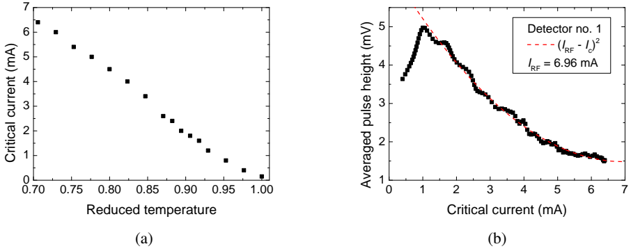
Fig. 6.12: (a) Temperature dependence of the critical current for detector no. 1. (b) Averaged pulse height measured in zero-bias operation mode with detector no. 1 depending on its critical current. The data can be interpolated by a square-law fit assuming flux flow.
