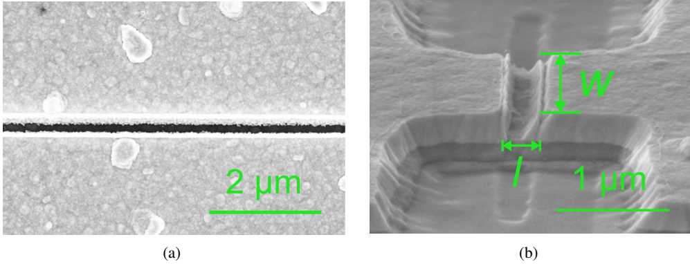
Fig. 5.8: SEM images of the YBCO THz detector fabrication: (a) slit in the gold metallization after etching with a width of 150 nm and (b) YBCO detecting element in the center of the antenna arms.
