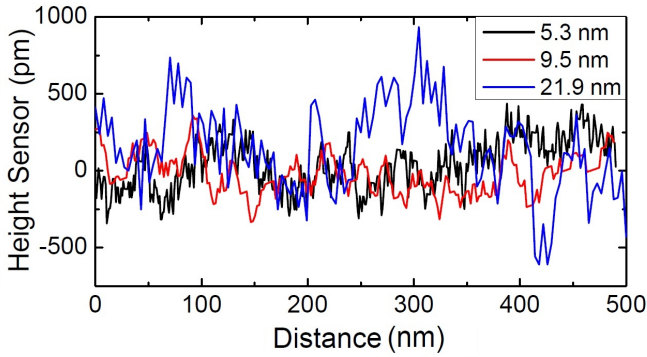
Fig. 4.11: AFM line scans for different CeO 2 film thicknesses.
