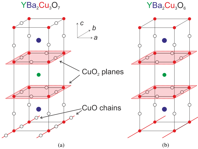
Fig. 3.1: YBCO unit cell: (a) orthorhombic \text{YBa}_2\text{Cu}_3\text{O}_7 phase and (b) tetragonal \text{YBa}_2\text{Cu}_3\text{O}_6 phase.
