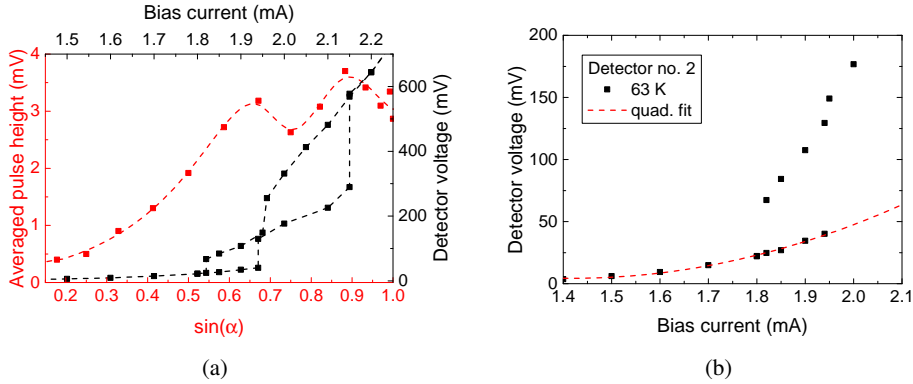
Fig. 6.11: Dependence of the zero-bias detector response on the I(V) curve for detector no. 2 at 63 K: (a) Comparison of the characteristics of the electrical-field dependence of the detector response with the I(V) curve above the critical current. (b) Quadratic fit of the I(V) characteristic at 63 K for low bias currents in the flux-flow regime.
