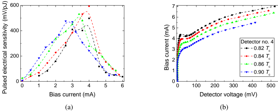
Fig. 7.3: (a) Electrical sensitivity of detector no. 4 measured at ANKA at different temperatures, and (b) corresponding I(V) characteristics of detector no. 4 at the same temperatures as in (a).
