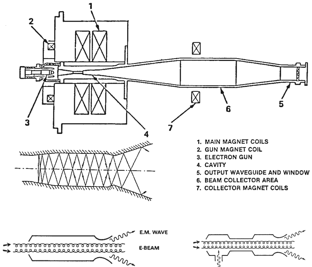
Fig. 1: Schematic of VARIAN CW gyrotron oscillator [14,19] and scheme of irregular waveguide cavities of gyromonotron oscillator (left) and two-cavity gyrokystron amplifier [361,362].
