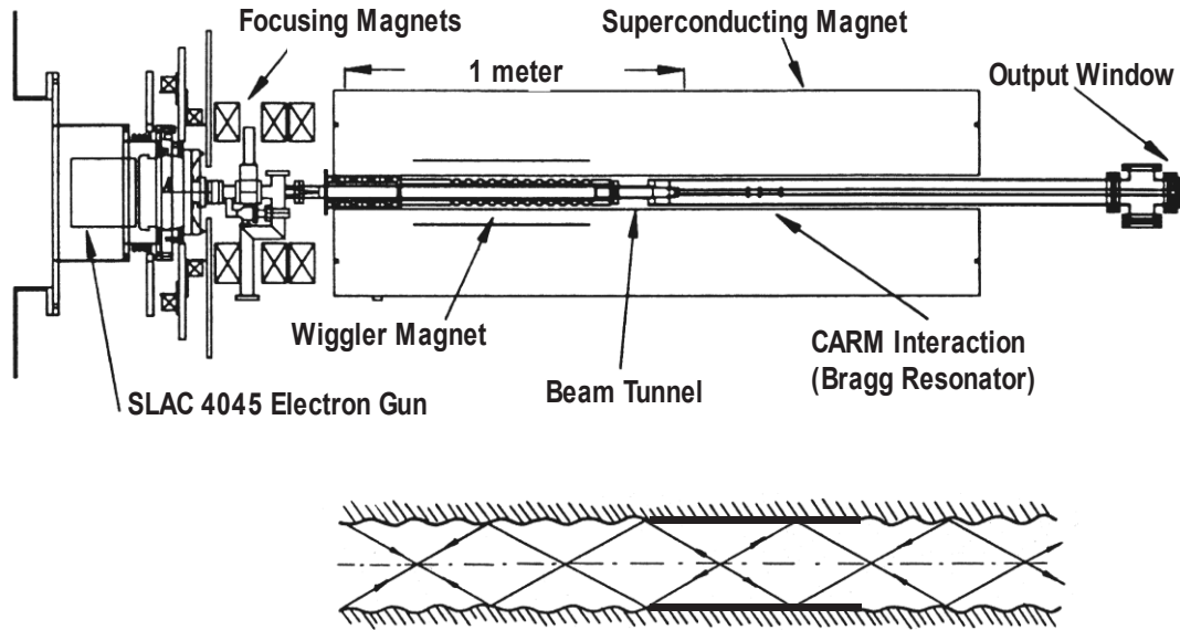
Fig. 7: Schematic of the long-pulse MIT CARM oscillator experiment [381] and scheme of a Bragg resonator [343].
