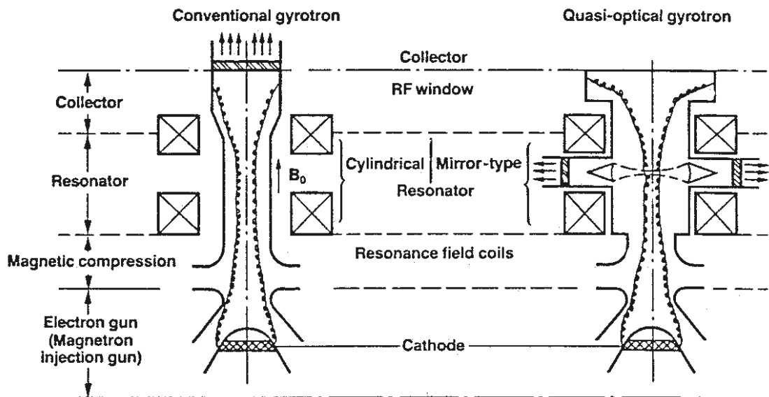
Fig. 2: Principle of a conventional gyrotron with cylindrical resonator and of a quasi-optical gyrotron with mirror resonator [95,96].
