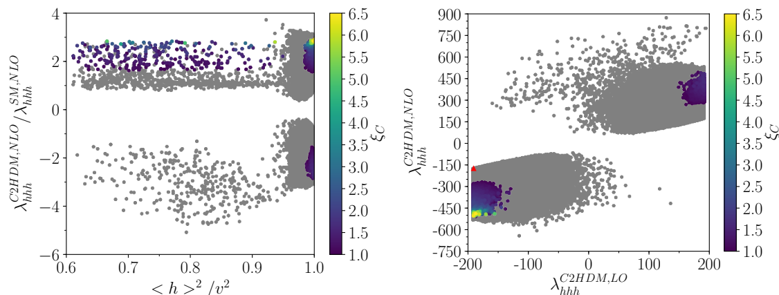
Figure 17. Type II, H_1 = h : left: the C2HDM trilinear Higgs self-coupling between three SM-like Higgs bosons h normalized to the SM value, at NLO, as function of the fraction of the VEV squared carried by h ; right: the NLO coupling versus the LO value. Grey: all points passing the constraints; colour: points with additionally \xi_c > 1 . The red triangle marks the SM point.
