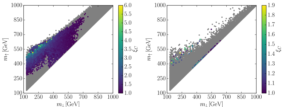
Figure 4. Type I, H_1 = h : the mass of the heavier versus the lighter non-SM-like Higgs boson. Left: CP-conserving and CP-violating points, right: only CP-violating points. Grey: points passing all the constraints; color: points with additionally \xi_c \geq 1 . The color code indicates the value of \xi_c .
