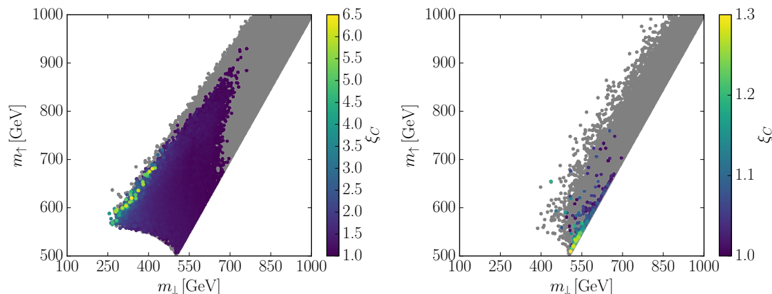
Figure 13. Type II, H_1 = h : the mass of the heavier versus the lighter non-SM-like Higgs boson. Left: CP-conserving and CP-violating points, right: only CP-violating points. Grey: points passing all the constraints; color: points with additionally \xi_c \geq 1 . The color code indicates the value of \xi_c .
