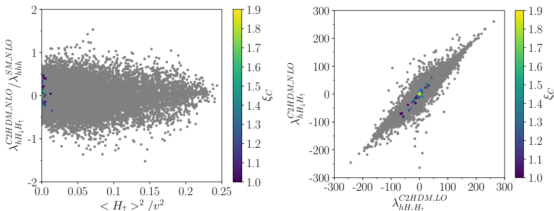
Figure 10. Type I, H_1 = h : left: the C2HDM trilinear Higgs self-coupling \lambda_{hH_\downarrow H_\uparrow} normalized to the SM value, at NLO, as a function of the fraction of the VEV squared carried by H_\uparrow . Right: the NLO C2HDM trilinear coupling \lambda_{hH_\downarrow H_\uparrow} versus the LO value. Grey: all points passing the constraints; colour: points with additionally \xi_c \geq 1 . Both plots: all 2HDM points.
