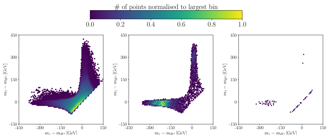
Figure 5. Type I, H_1 = h : the mass difference m_\uparrow - m_{H^\pm} versus m_\downarrow - m_{H^\pm} . The colour code shows the relative frequency of left: all points passing the constraints; middle: all points with a strong PT and CP conservation; right: all points with \xi_c \geq 1 and explicit CP violation.
