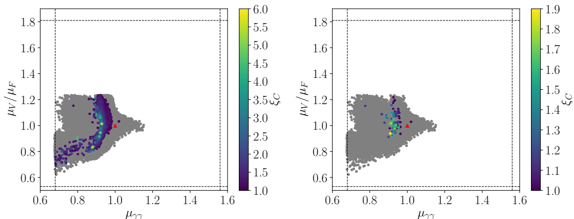
Figure 6. Type I, H_1 = h : \mu_V/\mu_F versus \mu_{\gamma\gamma} . Grey: all points passing the applied constraints, colour: all points with additionally \xi_c \geq 1 ; left: all 2HDM points, right: only C2HDM points. The red triangle marks the SM result.
