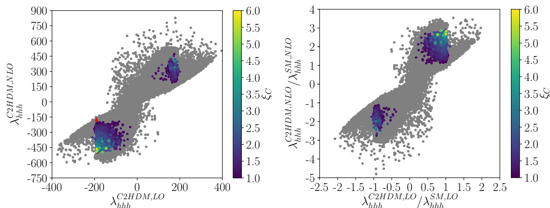
Figure 9. Type I, H_1 = h : left: the NLO C2HDM trilinear Higgs self-coupling between three SM-like Higgs bosons versus the LO value. The red triangle marks the SM point. Right: the ratio of the C2HDM trilinear Higgs self-coupling between three SM-like Higgs bosons and the SM counterpart at NLO versus the LO ratio. Grey: all points passing the constraints; colour: points with additionally \xi_c \geq 1 . Both plots: all 2HDM points.
