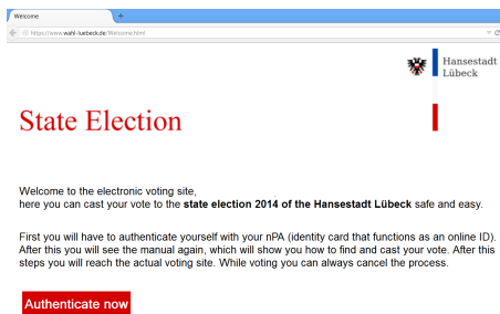
Figure 3: Welcome interface.
