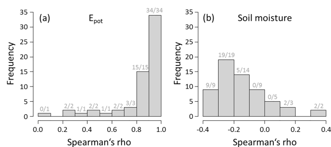
Figure 3. Histograms of temporal correlations between (a) E_{\text{pot}} and (b) soil moisture at each site with sap velocity for the 61 trees in the dataset. The small numbers in grey on top of the bars indicate how many of the correlations in the specific group are significant.
