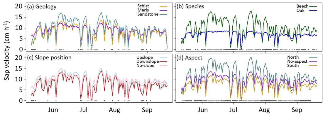
Figure 5. Differences between sap velocities depending on (a) geology, (b) species, (c) slope position and (d) aspect. Lines show the average dynamics of each class. Asterisks at the bottom of the panels indicate significant differences for that day according to Mann–Whitney U or Kruskal–Wallis tests at \alpha = 0.05 , for differences between the two or three categories, respectively.
