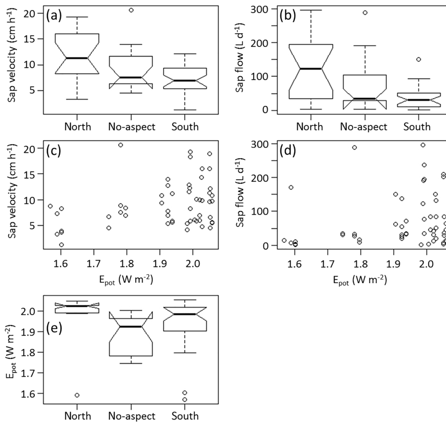
Figure A2. (a) Sap velocity and (b) sap flow values grouped according to aspect categories. (c) Sap velocities and (d) sap flow values of each tree with respect to E_{\text{pot}} at the tree location. (e) E_{\text{pot}} values at the tree locations values grouped according to aspect categories. Shown are temporal averages, for each tree (for sap velocity and sap flow) or each tree site (for E_{\text{pot}} ). The uncharacteristically high sap flow values are probably due to overestimation during the upscaling to tree-level transpiration and should be treated with caution; however, absolute values are not of interest here, rather relations and spatial patterns which should be robust.
