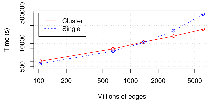
Figure 2.10: Time needed for creation of datasets with different numbers of edges. [17]
