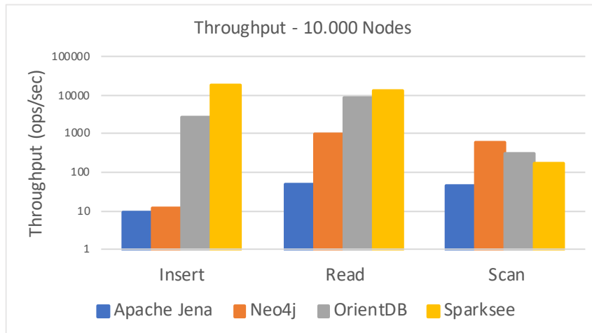
Figure 6.14: Throughput in operations/s of the different operations.
