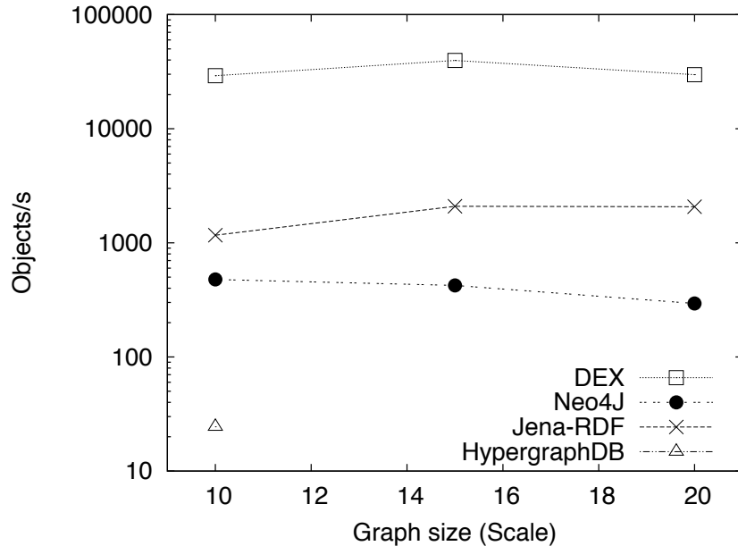
Figure 2.7: Throughput results of Dominguez-Sal et al. [16]
