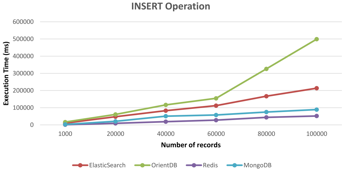
Figure 2.6: Time needed to insert different dataset sizes. [12]
