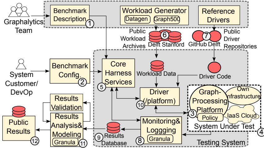
Figure 2.3: The architecture of the Graphalytics benchmark. [18, p. 11]
