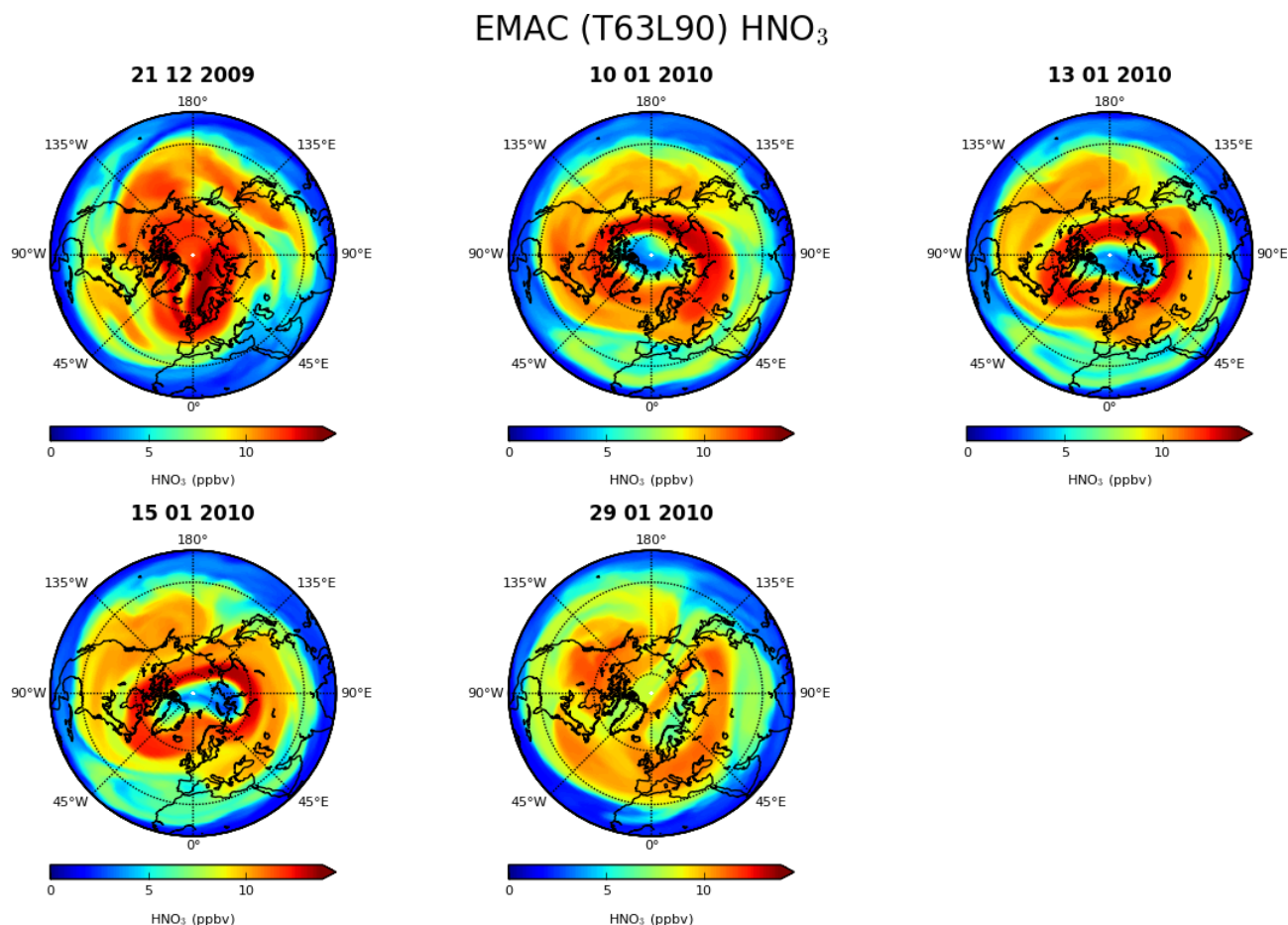
Figure 1. Distribution of HNO 3 as simulated with EMAC for 21 December 2009, 10, 13, 15, and 29 January 2010 at 34 hPa ( \approx 21 km).
