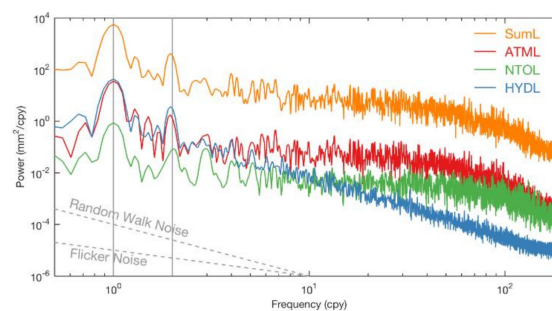
Figure 11. Stacked power spectra of the vertical displacements due to ATML, NTOL, HYDL, and SumL for the selected 208 CMONOC-II stations. The stacked power spectrum of SumL has been shifted upward for clarity (by a factor of 100). Vertical gray lines indicate the annual and semiannual oscillations.
