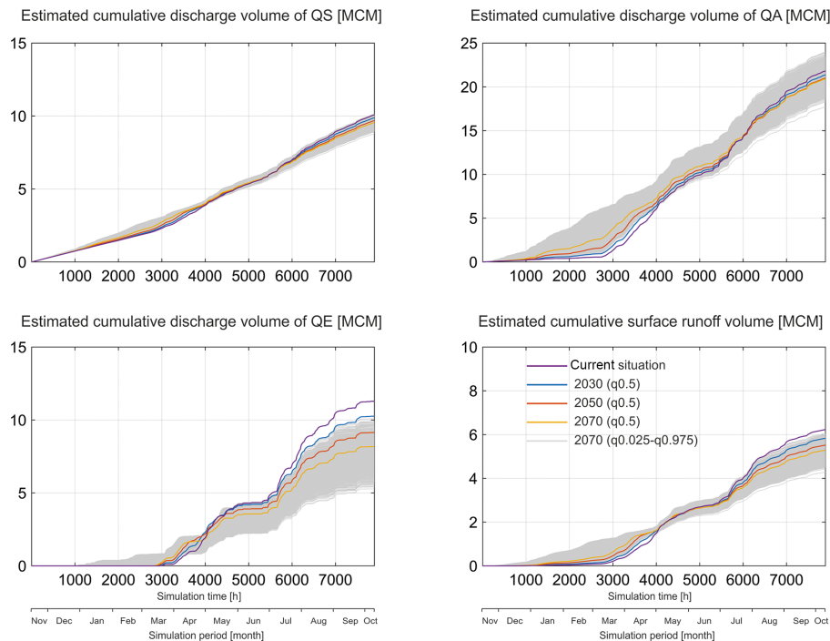
Figure 9. Impacts of the median climate scenarios ( q0.5 ) for years 2030, 2050 and 2070 as well as the uncertain climate scenarios (1000 random sampled combinations) for 2070 on the simulated discharge of QS, QA, QE and surface runoff from the non-karst area.
