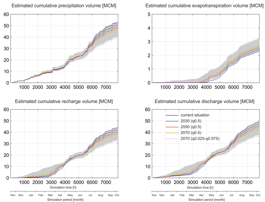
Figure 7. Impacts of the median climate scenarios ( q_{0.5} ) for years 2030, 2050 and 2070 as well as the uncertain climate scenarios (1000 random sampled combinations) for 2070 on the simulated precipitation, evapotranspiration, recharge and discharge for the studied catchment.
