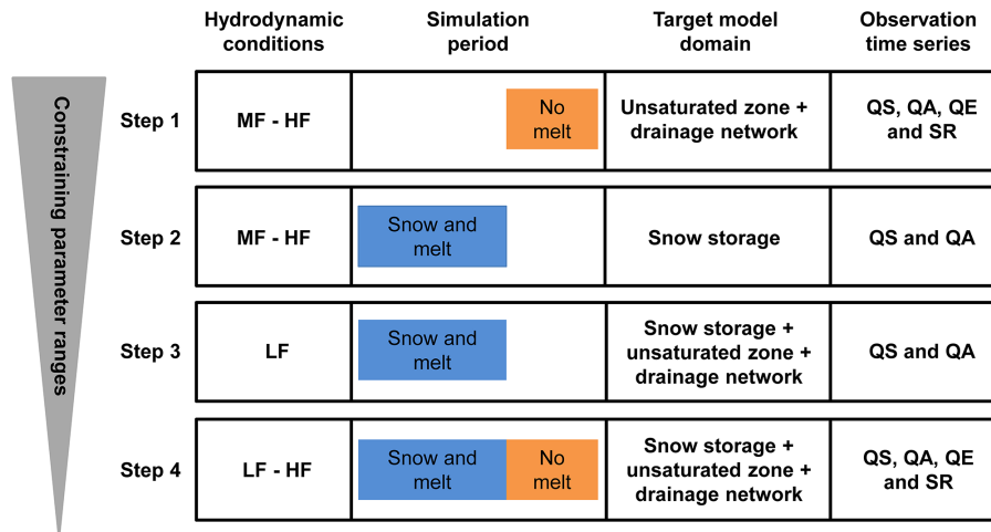
Figure 3. Strategy for the multi-step model calibration, where LF, MF and HF are for low-, medium- and high-flow conditions, respectively.
