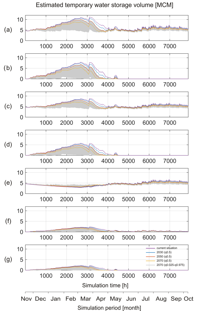
Figure 8. Impacts of the median climate scenarios ( q_{0.5} ) for years 2030, 2050 and 2070 as well as the uncertain climate scenarios (1000 random sampled combinations) for 2070 on (a) the simulated water storage of the whole catchment, (b) the simulated snow storage of the whole catchment, (c) the simulated water storage of the karst area, (d) the simulated snow storage of the karst area, (e) the simulated water storage of the karst aquifer, (f) the simulated water storage of the non-karst area and (g) the simulated snow storage of the non-karst area.
