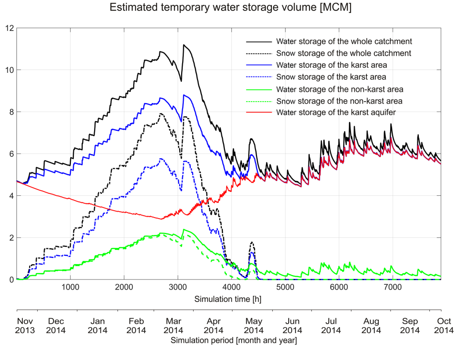
Figure 6. Estimated temporary water storage volumes for the whole catchment, karst area, non-karst area and karst aquifer for the period November 2013–October 2014 on an hourly time step in million cubic meters (MCM).
