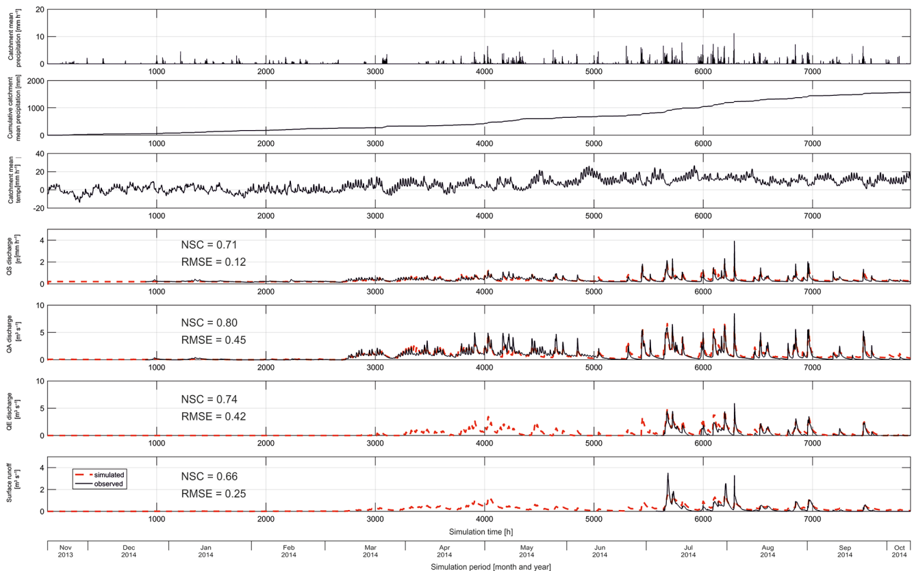
Figure 4. Observed and simulated discharge of four spatially distributed model outlets QS, QA, QE and SR using the best calibrated model parameter set for the period November 2013–October 2014. Additionally, the mean catchment precipitation and temperature for the same period are shown.
