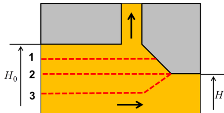
Figure 9. The conditional boundaries of the metal flows for the three possible PFM modes: Mode 1: \bar{P}_{BP} < \bar{P}_{BP1} ; Mode 2: \bar{P}_{BP1} \leq \bar{P}_{BP} \leq \bar{P}_{BP2} ; Mode 3: \bar{P}_{BP} > \bar{P}_{BP2} .
