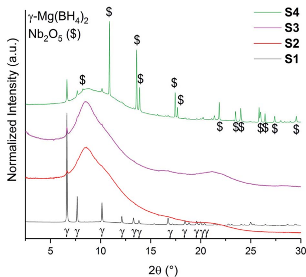
Fig. 1 SR-PXD data of \gamma -Mg(BH 4 ) 2 samples (S1–S4) at RT. All samples have been normalized to its maximum intensity and are shifted on the y-axis for better visibility. \lambda = 0.7454 \text{ \AA} .
