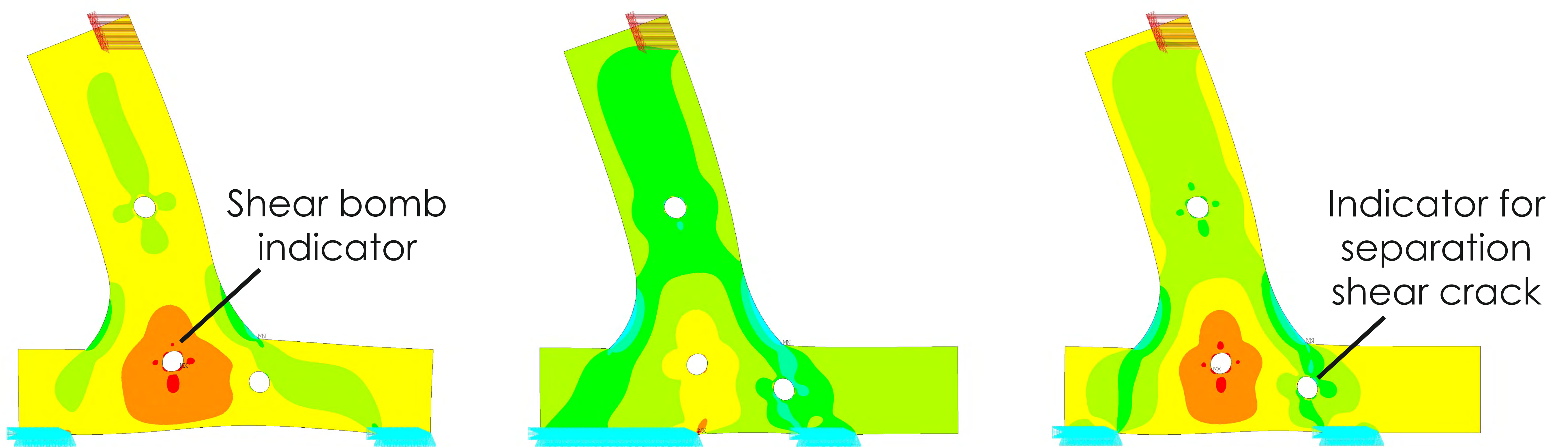
Plots of shear stresses \sigma_{xy}
