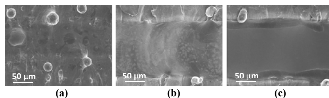
Fig. 2. SEM images of surfaces treated with cw laser: (a) 5 W and 90 \text{ mm s}^{-1} : no significant effect on the surface; (b) 20 W and 20 \text{ mm s}^{-1} : presence of cracks; (c) 25 W and 90 \text{ mm s}^{-1} : laser ablation.
