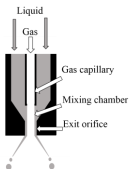
Fig. 1: Scheme of the used ACLR atomizer. ( l_{\text{mixing chamber}} = 2.4 \text{ mm} , l_{\text{exit orifice}} = 1.5 \text{ mm} , d_{\text{exit orifice}} = 1.5 \text{ mm} )
