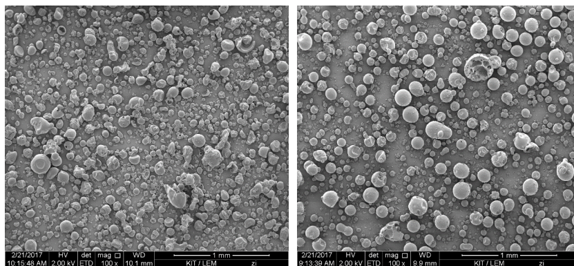
Fig. 3: Scanning electron microscope images of the industrially produced reference powder (left) and of the powder produced in the pilot scale process with ACLR atomizer (right) [15] .
