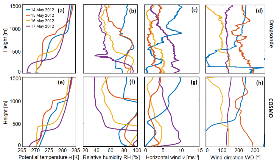
Figure 2. (a, e) Potential temperature, (b, f) relative humidity, (c, g) wind speed, and (d, h) wind direction for the four investigated cases. The dropsonde data are shown in the first row (a–d) and the 2 h domain-averaged profiles after spin-up time of the simulations are shown in the second row (e–h). Dropsondes were released closest to the imaging spectrometer measurements.
