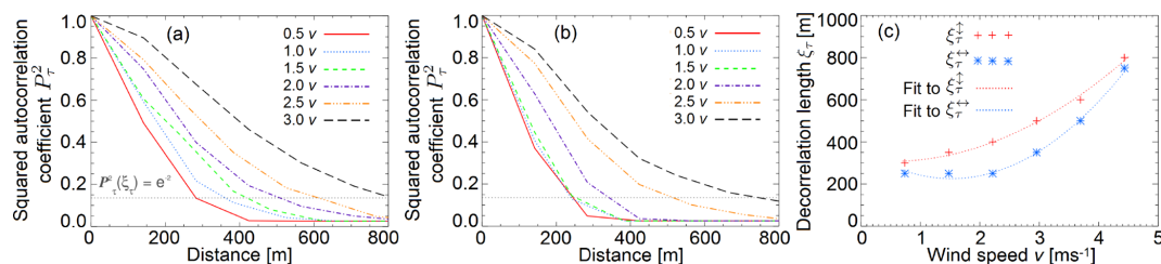
Figure 9. The six cases of different wind speed calculated 1-D autocorrelation functions (a) along and (b) across the main structures are identified in Fig. 8g–l. The grey dotted line marks the threshold of P_{\tau}^2(\xi_{\tau}) = e^{-2} . (c) From (a) and (b) derived discrete values for the decorrelation lengths \xi_{\tau}^{\downarrow} and \xi_{\tau}^{\leftrightarrow} as a function of wind speed v (symbols). Additionally included are fits derived from Eqs. (5) and (6) (dotted lines).
