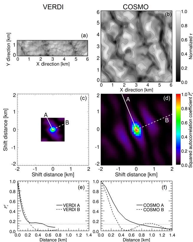
Figure 4. (a–b) Horizontal fields of normalized \tau_{\text{meas}} (VERDI) and \tau_{\text{sim}} (COSMO) for the case on 15 May 2012. (c–d) Two-dimensional autocorrelation coefficients P_{\tau,\text{meas}}^2 and P_{\tau,\text{sim}}^2 , calculated for fields of \tau displayed in panels (a) and (b). (e–f) One-dimensional autocorrelation coefficients along (straight white line marked in panels c and d) and across (dashed white line marked in panels c and d) predominant directional structure. The grey dotted line illustrates the threshold for the estimation of \xi_{\tau}^{\updownarrow} and \xi_{\tau}^{\leftrightarrow} .
