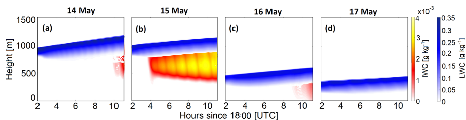
Figure 3. Domain averages of LWC (blue color scale) and IWC (red–yellow color scale) of the four simulations during the VERDI campaign. Please note the different color scale for the IWC in panel (d).
