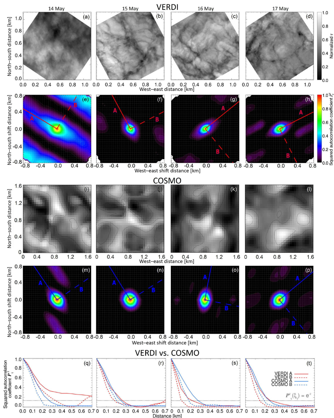
Figure 7. (a–d) Exemplary selected sections of fields of \tau_{\text{meas}} observed during VERDI from 14 to 17 May 2012. (e–h) Mean 2-D autocorrelation coefficients P_{\tau_{\text{meas}}}^2 derived for fields of \tau_{\text{meas}} from VERDI. (i–l) Exemplary selected fields of \tau_{\text{sim}} simulated with COSMO (50 m spatial resolution) for the VERDI cases from 14 to 17 May 2012. (m–p) Mean 2-D autocorrelation coefficients P_{\tau_{\text{sim}}}^2 derived for fields of \tau_{\text{sim}} . (q–t) Decorrelation length \xi_{\tau} along strongest (straight blue and red lines) and weakest (dashed blue and red lines) extents of 2-D autocorrelation coefficients derived from P_{\tau_{\text{meas}}}^2 in panels (e)–(h) and P_{\tau_{\text{sim}}}^2 in panels (m)–(p), respectively.
