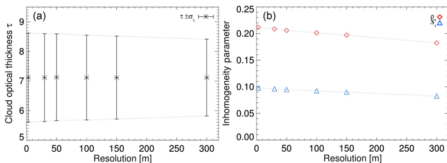
Figure 6. Comparison of (a) mean and standard deviation and (b) inhomogeneity parameters ( \rho and S ) as a function of spatial resolution for the fields of \tau_{\text{meas}} illustrated in Fig. 5a–e.
