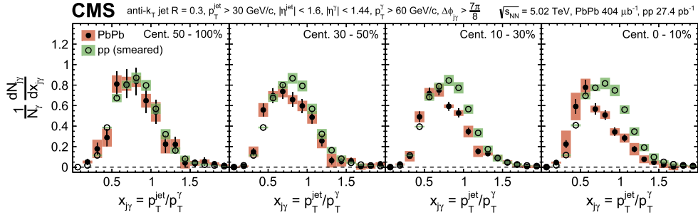
Fig. 6. The centrality dependence of x_{j\gamma} of photon+jet pairs normalized by the number of photons for PbPb (full markers) and smeared pp (open markers) data. The vertical lines (bands) through the points represent statistical (systematic) uncertainties.
