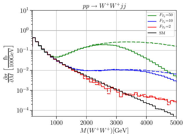
Fig. 3 Cross sections differential in the diboson invariant mass for the process pp \rightarrow W^+W^+jj . The solid black line shows the SM differential cross section, the green, blue and red lines the cross sections with anomalous couplings F_{T_i} = 50 \text{ TeV}^{-4} , F_{T_i} = 10 \text{ TeV}^{-4} and F_{T_i} = 2 \text{ TeV}^{-4} for i = 0 (upper panel), i = 1 (middle panel), and i = 2 (lower panel), respectively. Solid: unitarized; dashed: naive result. Cuts: M_{jj} > 500 \text{ GeV} , \Delta\eta_{jj} > 2.4 , |\eta_j| < 4.5 , p_T^j > 20 \text{ GeV}
