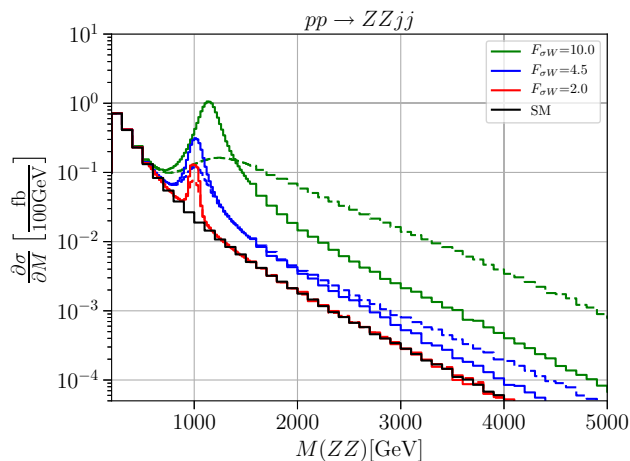
Fig. 4 Cross sections differential in the diboson invariant mass for the process pp \rightarrow ZZjj . The solid black line shows the Standard Model differential cross section, the green, blue and red lines the cross sections with a scalar resonance with mass m_\sigma = 1 TeV and coupling of F_{W\sigma} = 10.0 \text{ TeV}^{-1} , F_{W\sigma} = 4.5 \text{ TeV}^{-1} and F_{W\sigma} = 2.0 \text{ TeV}^{-1} , respectively. Solid: unitarized; dashed: naive result. Cuts: M_{jj} > 500 \text{ GeV} , |\eta_{jj}| > 2.4 , |\eta_j| < 4.5 , p_T^j > 20 \text{ GeV}
