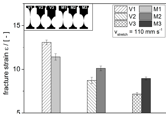
Figure 6. Fracture strain \epsilon results obtained from sample stretching experiments measured with the capillary breakup elongation rheometer (CaBER) device at v_{stretch} = 110 \text{ mm s}^{-1} stretching speed. Exemplary pictures of stretched and broken filaments for vehicles and silver pastes are shown inset. Patterned bars correspond to vehicles, filled bars represent silver pastes.
