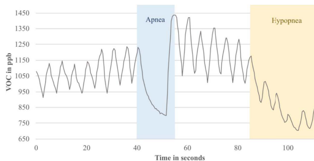
Figure 4. Graph for sleep disorder detection (x-axis: time [s], y-axis: VOC [ppb]). Apnea event marked blue, hypopnea yellow.
