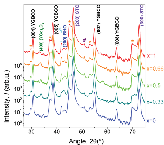
Fig. 3 XRD patterns of Y_{1-x}Gd_xBa_2Cu_3O_{7-\delta} + 12\% BHO films grown with optimized processing parameters. The peaks marked with * and # come from the experimental setup ( K_\beta filter and X-ray source, respectively).
