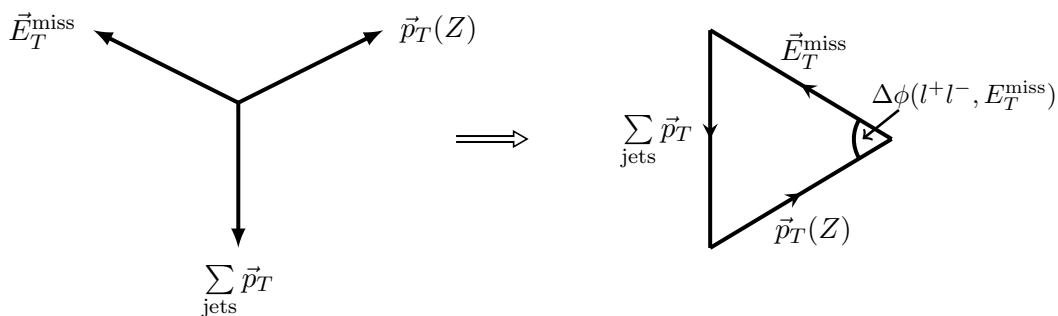
Figure 3. Sketch of different components of dilepton plus E_T^{\text{miss}} events in the transverse plane; the dilepton system recoils against the missing energy and the vector sum of hadronic p_T . Conservation of transverse momentum implies the vectors form a closed triangle, which can be defined by the lengths of two sides and the enclosed angle, or by the lengths of all three sides.
