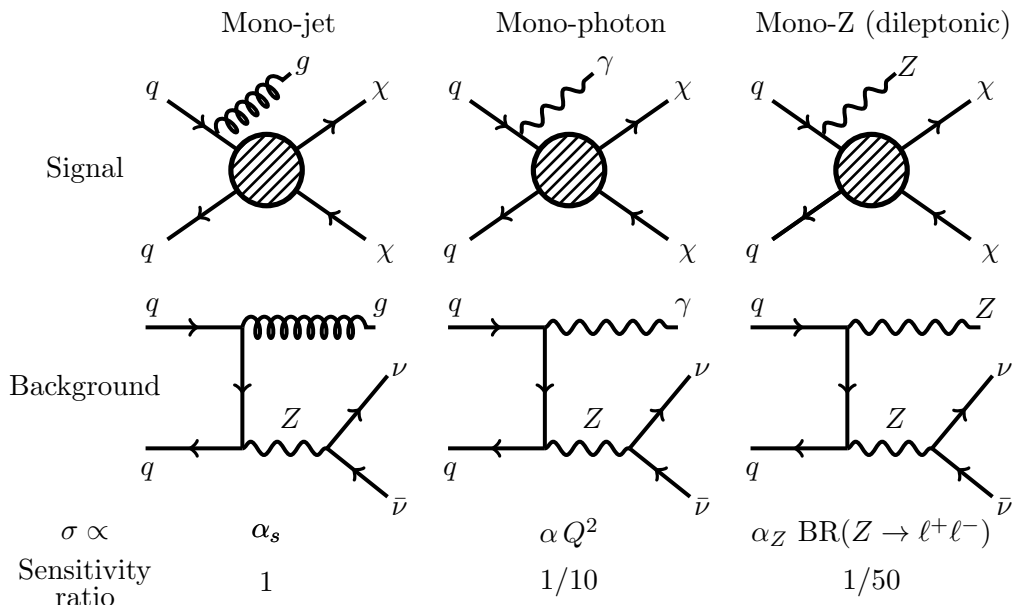
Figure 1. Relative signal sensitivity in three main mono- X channels. Since the cross sections for each signal and its irreducible background scale in the same way, if we assume the relative efficiency for the signal and background processes are the same over each of the different channels, the naive relative significance, computed as S/\sqrt{B} , scales as \sqrt{\alpha_s} : Q\sqrt{\alpha} : \sqrt{\alpha_Z \text{BR}(Z \rightarrow \ell^+\ell^-)} . However this argument does not account for systematic uncertainties, which we expect will grow at higher centre-of-mass energy.
