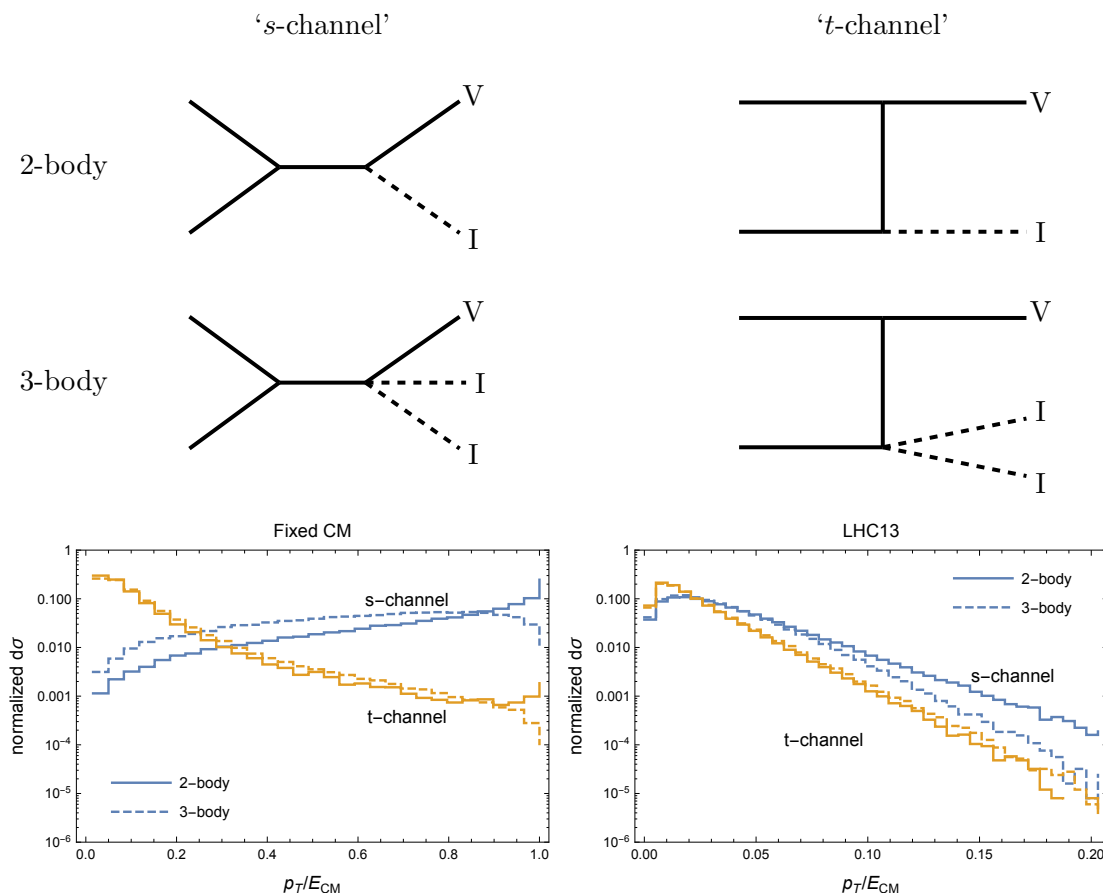
Figure 5. Normalized MET distributions for ‘ s -channel’ and ‘ t -channel’, 2- and 3-body topologies, with visible final state V and invisible states I . The 2-body t -channel topology corresponds to the irreducible SM di- Z background, as well as \chi\bar{\chi}Z production via an on-shell mediator. A compressed dark state produced instead via an off-shell gauge boson mediator, as it is here, is a 3-body, t -channel process.
