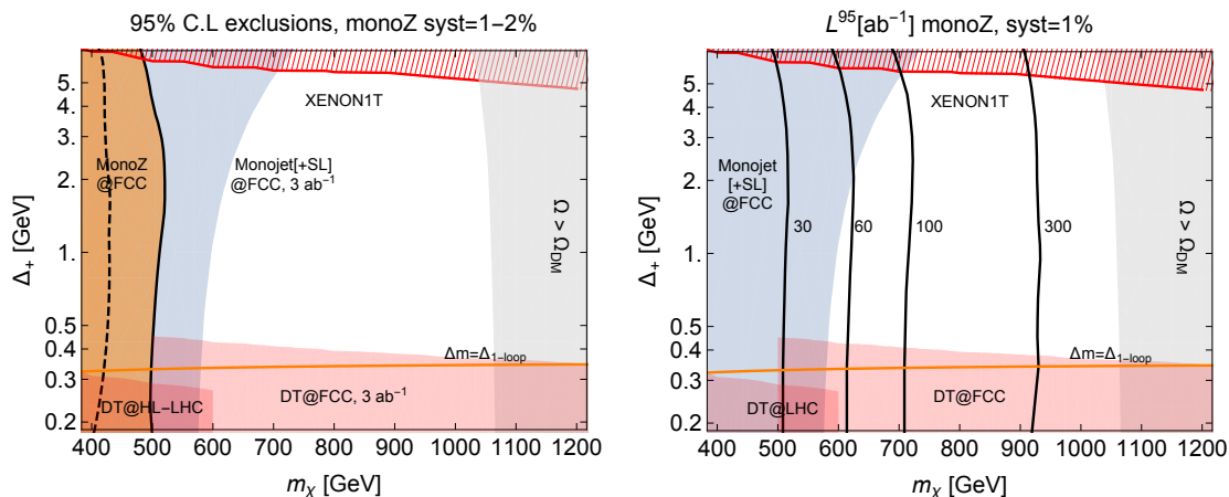
Figure 8. Higgsino parameter space covered by the existing studies and the proposed mono-Z search. (Left panel) The 95% CLs exclusion for our dileptonic mono-Z search, for 30 ab -1 of integrated luminosity at FCC-hh, and a background systematic uncertainty of 1% (solid black line) and 2% (dashed black line). Note that the other collider searches shown use a lower luminosity of 3 ab -1 . For more details see caption of figure 7 and text. (Right panel) Contours of luminosity required for 95% CLs exclusion, L^{95} , for 1% systematic uncertainty in the background.
