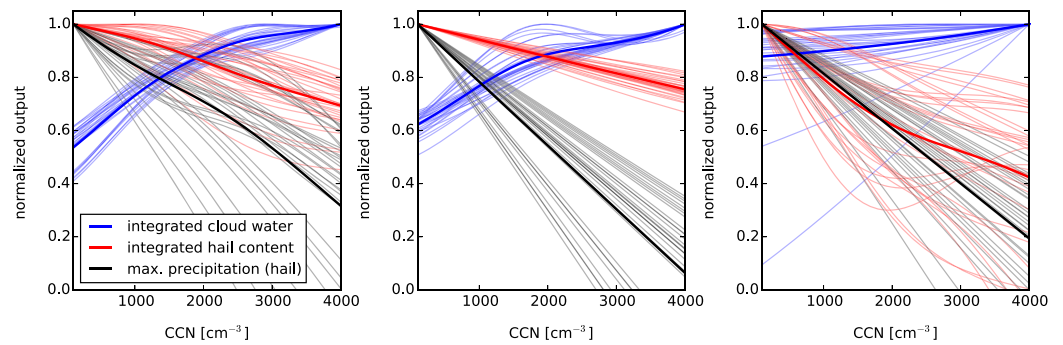
Figure 7. Sensitivity of mean integrated cloud water, mean integrated hail, and precipitation by hail to variations in the cloud condensation nuclei concentration for (a) the warm bubble setup, (b) the cold pool setup, and (c) the orography setup. Thin lines represent the results for 32 different environmental conditions (regimes), and the bold line denotes the mean. CCN = cloud condensation nuclei.
