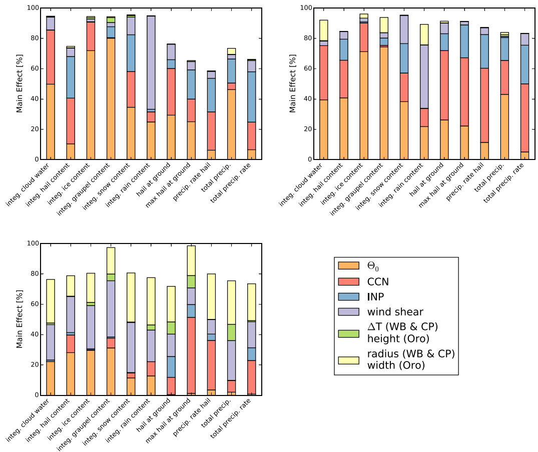
Figure 4. Bar plot of the main effect for vertically integrated hydrometeor masses and precipitation of cloudy grid points when (a) a warm bubble, (b) a cold pool, and (c) a mountain ridge is used as trigger mechanism. CCN = cloud condensation nuclei; CP = cold pool; INP = ice-nucleating particles; WB = warm bubble.
