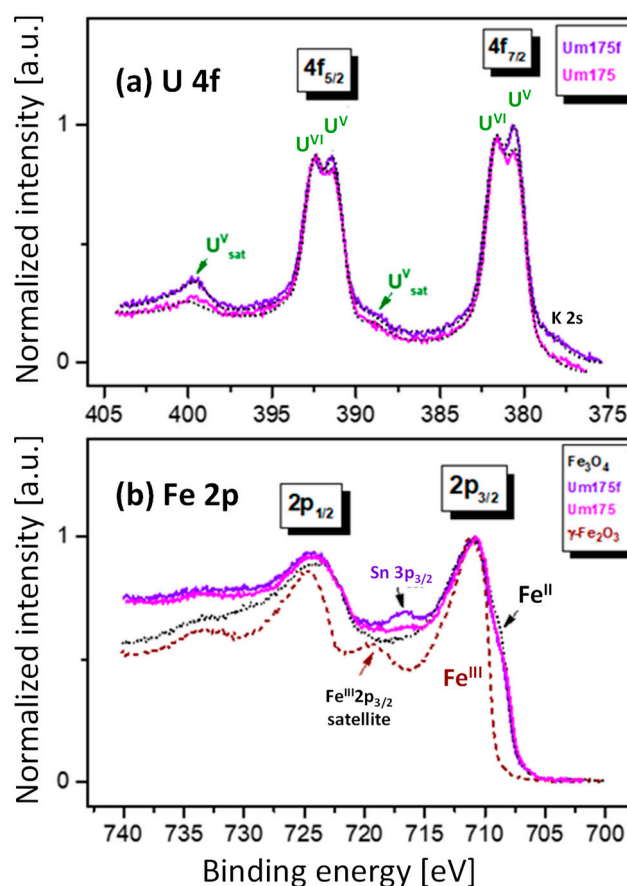
Figure 9. XP spectra of U(VI) reacted magnetite - (a) U 4f 7/2,5/2 doublet of Um175f (blue) and Um175 (violet); (b) Fe 2p 3/2,1/2 doublet of stoichiometric Fe 3 O 4 (dots), Um175f, Um175 and γ-Fe 2 O 3 (dashes).
