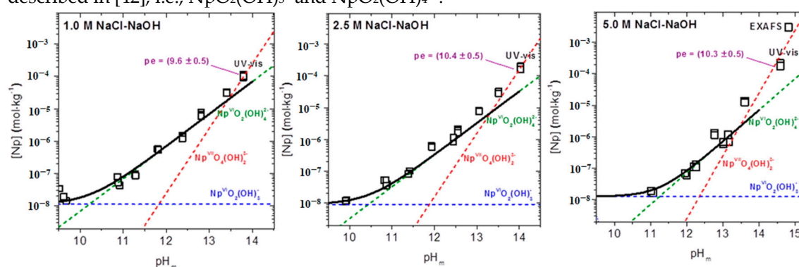
Figure 2. Experimental solubility data of \text{Na}_2\text{Np}_2\text{O}_7(\text{cr}) in 1.0, 2.5 and 5.0 M NaCl–NaOH solutions, as reported in [Error! Bookmark not defined.] and determined in this work. Solid lines correspond to the solubility of \text{Na}_2\text{Np}_2\text{O}_7(\text{cr}) calculated with the thermodynamic and activity models reported in [Error! Bookmark not defined.] for Np(VI). Blue and green dashed lines correspond to Np(VI) aqueous speciation underlying the solubility of \text{Na}_2\text{Np}_2\text{O}_7(\text{cr}) . The red dashed line indicates the contribution of the Np(VII) species \text{NpO}_4(\text{OH})_2^{3-} to the solubility as proposed in this work. The figures indicate also those samples for which UV-vis [Error! Bookmark not defined.] and XAFS (present work) spectra of the supernatant solution were collected.
