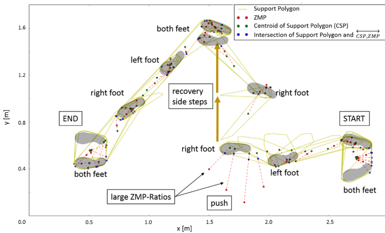
Figure 4.14: Top view of the support polygon (yellow), its centroid (green), the ZMP (red) and the intersection (blue) of the line (dashed red) defined by the ZMP and the centroid with the support polygon for every 10^{\text{th}} frame of a motion in which the human subject walked forward, was pushed from the left and then continued to walk. Scale in meters (adapted from [Steffan et al. 2017], © 2017 IEEE).
