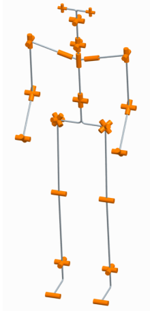
(b) Kinematic structure of the ARMAR-4 humanoid robot
