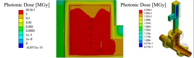
Fig. 5. Absorbed \gamma dose spatial distribution in a UPC slice detail (left) and in the valve (right).
