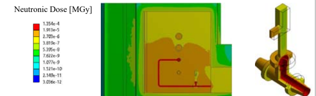
Fig. 7. Absorbed neutron dose spatial distribution in a UPC slice detail (left) and in the valve (right).
