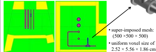
Fig. 3. Sections of the MCNP model of the UPC: a) Toroidal-Radial section; b) Poloidal-Radial section.
