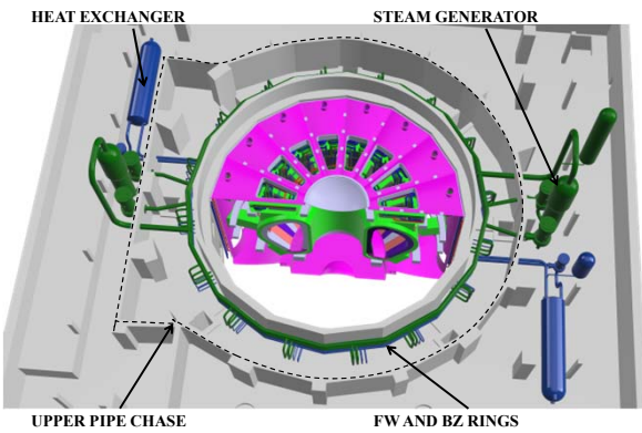
Fig. 1. View of DEMO PHTS in the UPC.
