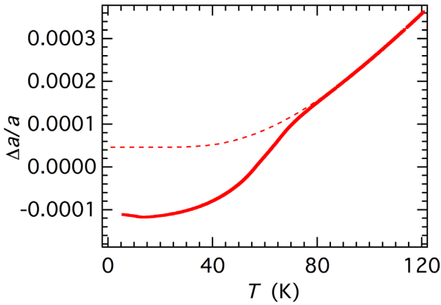
Figure A5. Relative length change of single crystal of \text{Ba}(\text{Fe}_{0.955}\text{Co}_{0.045})_2\text{As}_2 ([48]) with a fit of equation (3) to the data above T_S (dashed line): a_1 = -8.37 \times 10^{-4} , a_2 = 7.76 \times 10^{-6} , \Theta_s = 113.8\text{K} .
