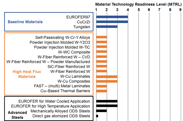
Fig 6: MTRL of baseline materials and advanced steels and high heat flux materials
