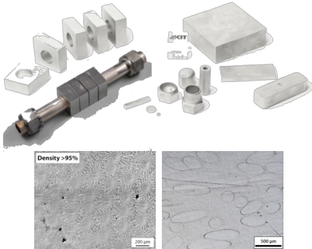
Fig 4: Various tungsten pieces produced via PIM and the produced mock-up after exposure to 20 MW/m 2 (top); microstructure of long and short fiber reinforced tungsten (bottom)
