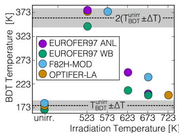
Fig 1: Temperatures of brittle to ductile transitions (BDT) in several fusion steels. A model [12] based on the analysis of screw dislocation mobility suggests that the BDT temperature doubles if irradiation is performed at relatively low temperature.
