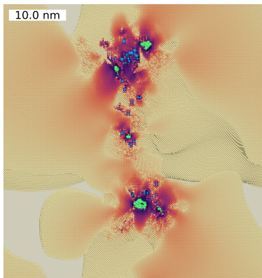
Fig. 7. A diagonal component of the stress tensor, plotted using a colour scheme reflecting the magnitude of stress, in the vicinity of radiation defects produced by a 150 keV neutron impact in pure tungsten. The green and blue spheres are the interstitial and vacancy defects, respectively, identified using the Wigner-Seitz cell analysis (image courtesy of A.E. Sand, [33]).
