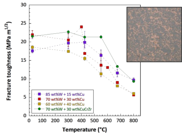
Fig 5: Fracture toughness of W-particle reinforced Cu and CuCrZr; microstructure of one of three industrially produced batches of W p -CuCrZr
