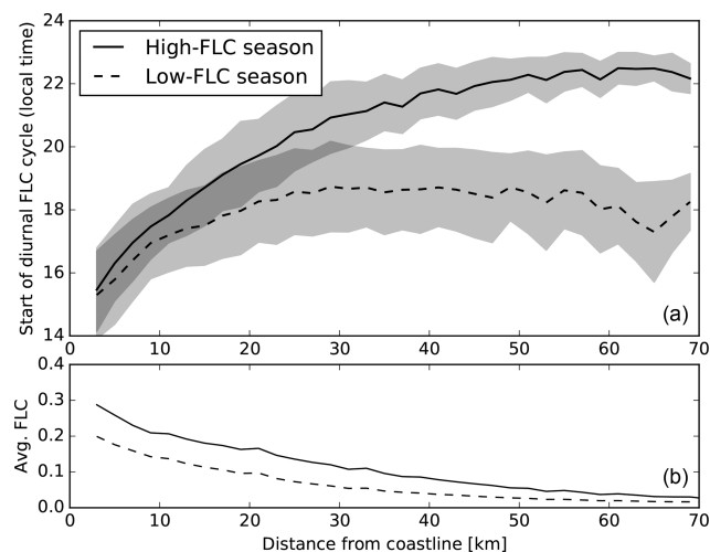
Figure 5. (a) Start of diurnal FLC cycle in the central Namib as a function of distance from the coastline. Two different seasons are shown: high-FLC season (September, October and November) and low-FLC season (April, May and June). Shaded area illustrates mean \pm 1 standard deviation. (b) Average relative FLC occurrence frequency in the two seasons. The same pixels are considered as in panel (a) and averaged in 2 km distance bins ( x axis).
