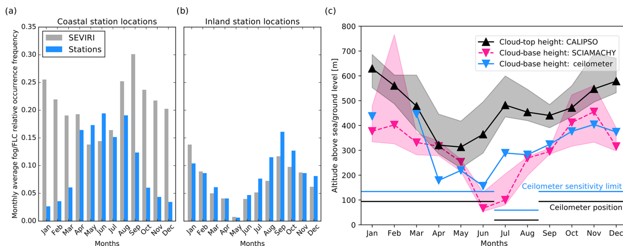
Figure 3. Monthly averaged relative fog/FLC occurrence frequency at locations of coastal (a) and inland stations (b) as defined in Fig. 1b. SEVIRI observations (2004–2017) are illustrated by grey bars; station measurements of ground fog (2015–2017) are in blue. (c) Medians, 25th and 75th percentiles of monthly averaged CBH and CTH in the central Namib based on SCIAMACHY (above ground level; 22.5–24.0° S and 14.25–15.5° E; 2003–2009) and CALIPSO (above sea level; 22.5–24.0° S and 14.0–15.5° E; 2006–2017) observations, respectively. Ceilometer CBH observations (above sea level) are only available starting from September 2017. Ceilometer positions (Coastal Met from September to June and Swakopmund in July and August) and sensitivity limits are illustrated by thin horizontal lines and described in Sect. 2.4.
