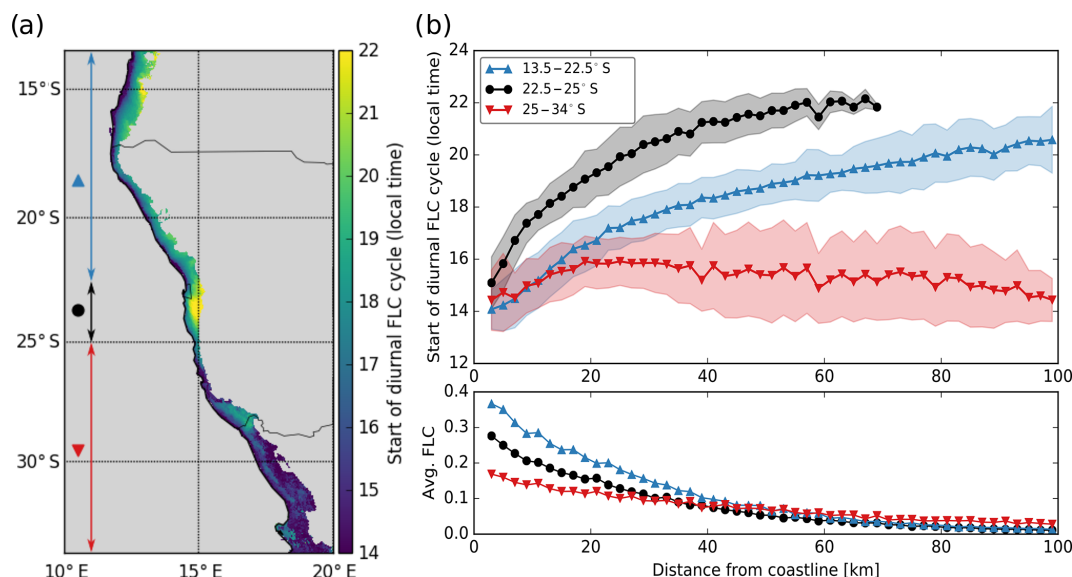
Figure 4. (a) The time of the start of the diurnal FLC cycle on pixel level. Pixels which are either more than 100 km removed from the coastline or feature a relative frequency of FLC occurrence of less than 5 % are not considered. The north–south-oriented arrows indicate the northern/southern extent of the three regions considered in panel (b), with colored markers illustrating their respective association. (b) Upper panel: the average timing of start of the diurnal FLC cycle as a function of average distance to the coastline. Shaded area illustrates mean \pm 1 standard deviation. Lower panel: average relative FLC occurrence frequency in the three subregions. The same pixels are considered as in panel (a) and are averaged in 2 km distance bins ( x axis).
