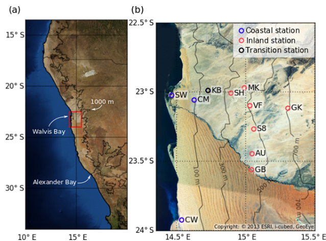
Figure 1. (a) An overview of the study area. The grey line represents 1000 m above sea level and approximates the transition from the low-lying coastal plains to the Great Escarpment that represents the eastern limit of the Namib desert. The red box in the Walvis Bay area highlights the central Namib, which is shown in more detail in panel (b): FogNet stations are illustrated by circles and are annotated with their respective IDs (full station names are given in the Appendix). Blue circles represent coastal and red circles inland stations as defined in this study (Sect. 2.4). The Kleinberg (KB) station is colored in black, as it is viewed to be at a transitional location not clearly belonging to either category.
