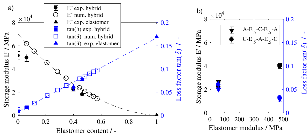
Figure 13. (a) Influence of elastomer content = (total thickness of both elastomer layers)/(thickness of specimen) for a (C-El s -A-El s -C) lay-up; (b) experimental results for the influence of the elastomer modulus.
