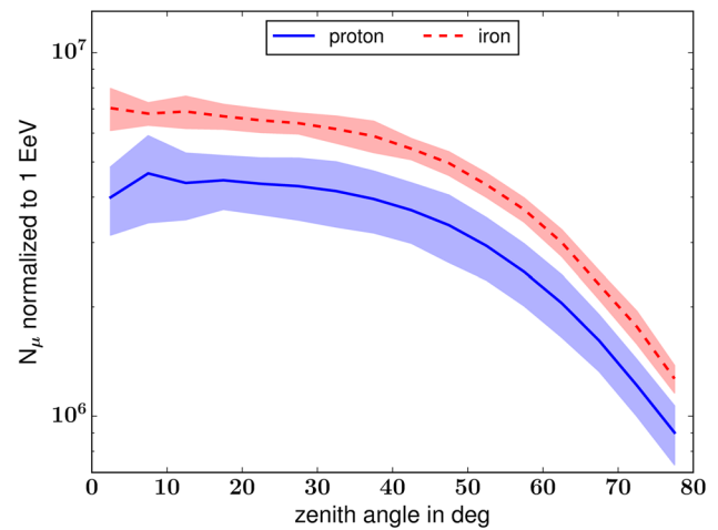
Fig. 1 Zenith angle dependence of the mean true number of muons at observation level ( E_\mu > 1 \text{ GeV} ). The number of muons is normalized to an energy of 10^{18} eV. For zenith angles larger than 40^\circ the traveled distance becomes large and a fraction of the muons decays during the shower development before reaching the observation level of 1552 m a.s.l. As also in the following figures, the lines and their surrounding bands denote the mean values and the standard deviations
