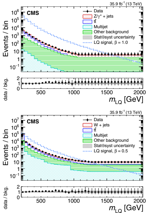
FIG. 7. Data, background, and expected signal yields after applying the final selection criteria for the eejj (left) and e\nu jj (right) channels. “Other background” includes diboson, single top quark, and W + jets (for the eejj channel) or Z/\gamma^* + jets (for the e\nu jj channel). The bin contents are correlated, because events selected for higher-mass LQ searches are a subset of those selected for lower mass searches.
