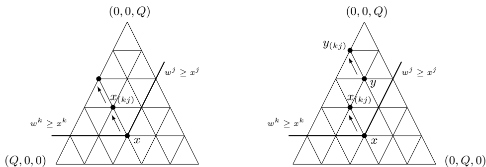
Fig. 1: Separable convexity
