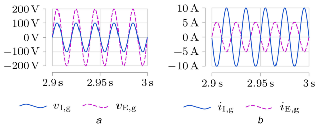
Fig. 5 Grid currents and voltages in the steady-state operation. Only one phase is shown (a) Phase voltages, (b) Phase currents
