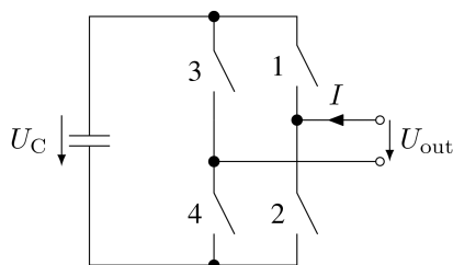
Fig. 1 Full-bridge cell
