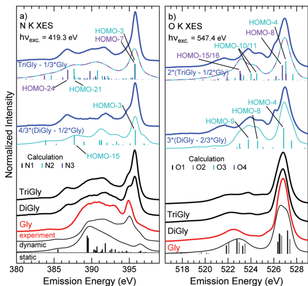
Fig. 2 (a) Non-resonant N K XES spectra of glycine (Gly), diglycine (DiGly), and triglycine (TriGly), normalized to area. Below the spectrum of glycine, two calculated spectra are shown (taken from ref. 26): a “static” electronic ground state DFT calculation and a “dynamic” calculation that includes molecular dynamics during the X-ray emission process. At the top (blue), weighted differences between the spectra of di-/triglycine and glycine are shown. Below the difference spectra, DFT calculations for the nitrogen atoms at the peptide bonds are shown as vertical bars (as calculated) and thin lines (broadened by Voigt profiles). (b) Non-resonant O K XES spectra of the three molecules, normalized to area. Below the spectrum of glycine, the DFT calculation for an isolated glycine zwitterion is depicted as black bars. Weighted difference spectra are again shown in blue, together with the DFT calculations for the oxygen atoms at the peptide bonds as vertical bars (as calculated) and thin lines (broadened by Voigt profiles).
