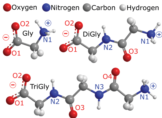
Fig. 1 Chemical structure of the zwitterions of glycine (Gly), diglycine (DiGly), and triglycine (TriGly). In all three structures, the amino group is protonated ( -NH_3^+ ) and the carboxyl group is deprotonated (forming carboxylate, COO^- ). Oxygen and nitrogen atoms are numbered and labelled.
