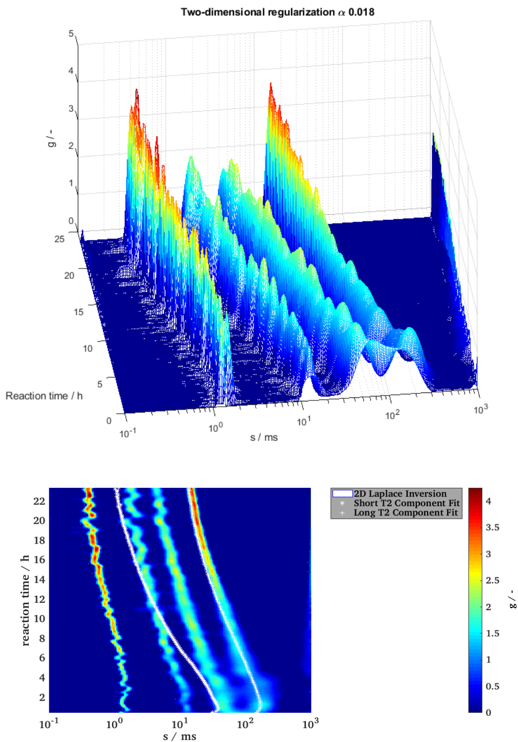
Figure 4: Top: Two-dimensional regularization for the Furfuryl alcohol polymerization. Bottom: Top-view of the spectra with added bi-exponential (white markers) fit.
