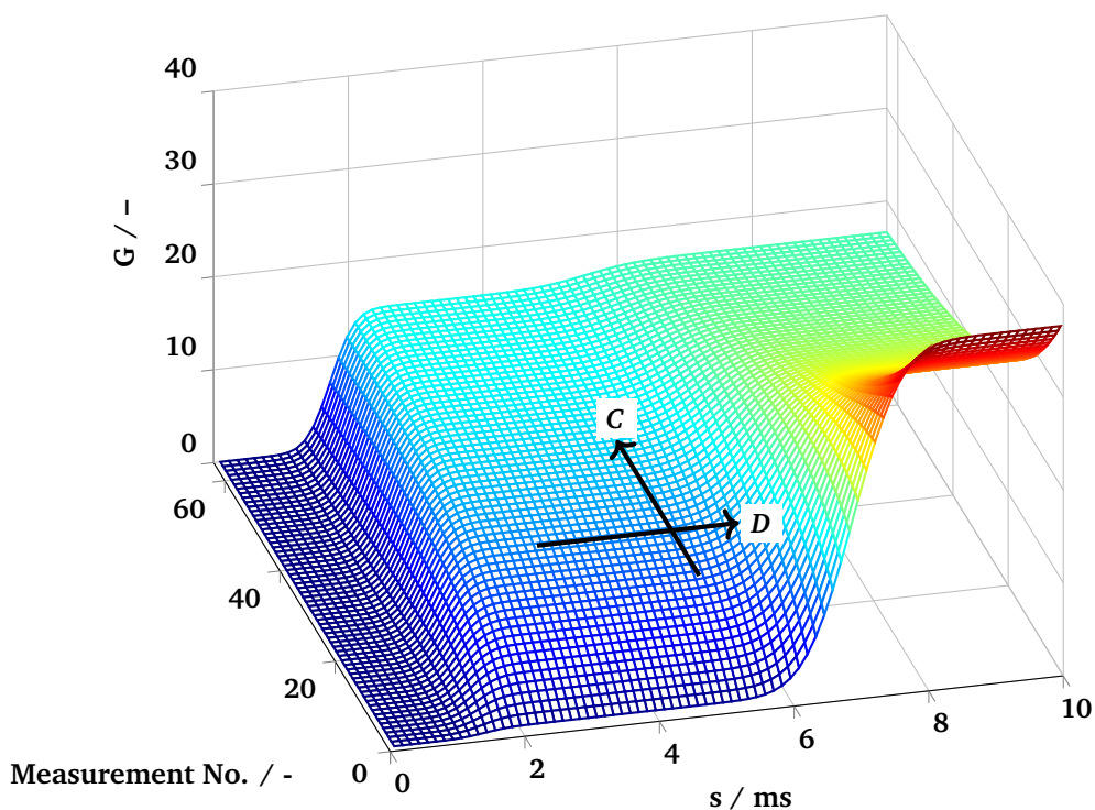
Figure 1: Cumulative sum of the simulated spectrum. The black arrows indicate the direction of the regularization by the matrices \mathbf{C} and \mathbf{D} .
