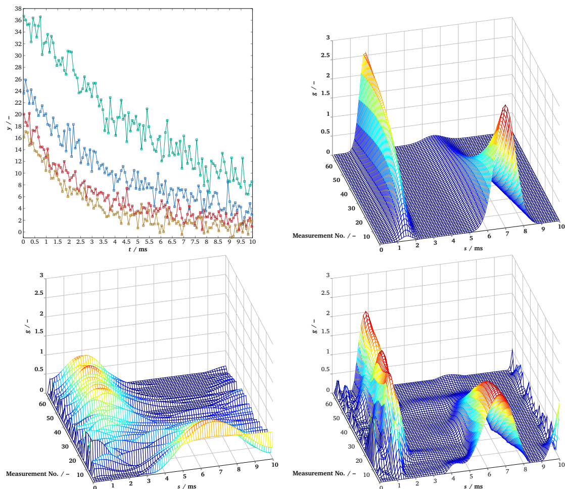
Figure 2: Top left: simulated measurement signal with noise; Top right: simulated spectrum; Bottom left: spectrum obtained with one-dimensional Laplace inversion of the simulated signal; Bottom right: spectrum obtained with two-dimensional Laplace inversion of the simulated signal.
