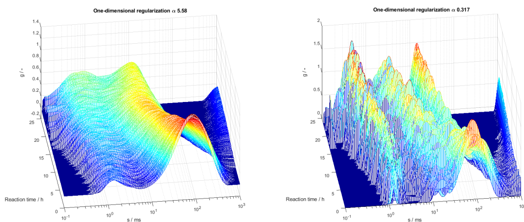
Figure 3: Left: Spectra of Furfuryl alcohol polymerization obtained with one-dimensional regularization and regularization parameter obtained with the L-curve method. Right: Spectra for the same sample using a lower regularization parameter.
