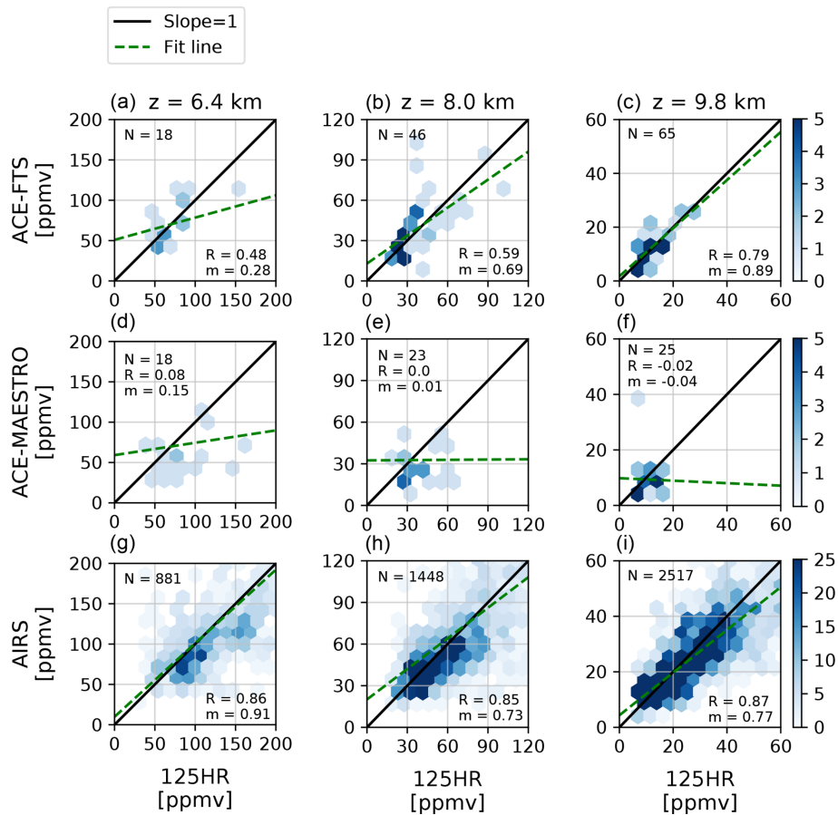
Figure 8. Correlation plots for the ACE-FTS, ACE-MAESTRO, and AIRS satellite measurements vs. 125HR. The number of points in a given hexagon is colour-coded to show the density of the points. The scale at each end of a row shows the colour map used for that row. Solid black lines are 1:1 reference lines (i.e. slope = 1); green dashed lines are lines of linear best fit. N is the number of coincident measurements for comparisons between the instruments at that altitude. R is the correlation coefficient. m is the slope of the best-fit line.
