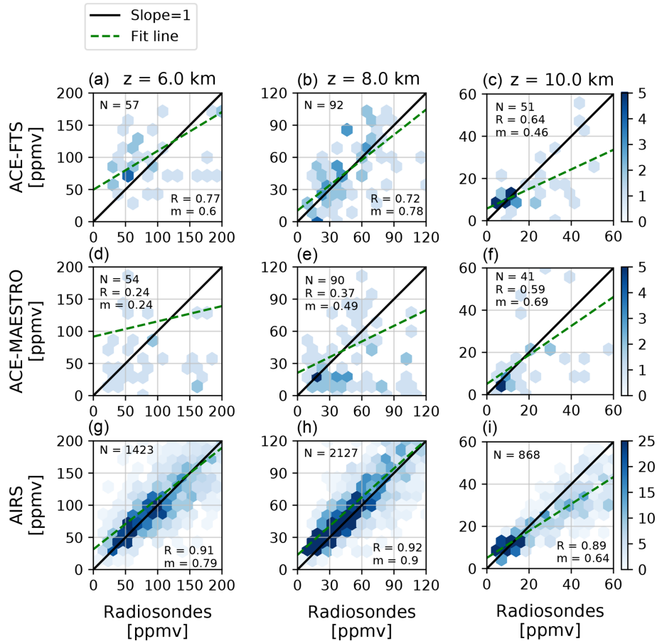
Figure 11. Same as Fig. 8, but with correlation plots for the ACE-FTS, ACE-MAESTRO, and AIRS satellite measurements vs. the Eureka radiosondes.
