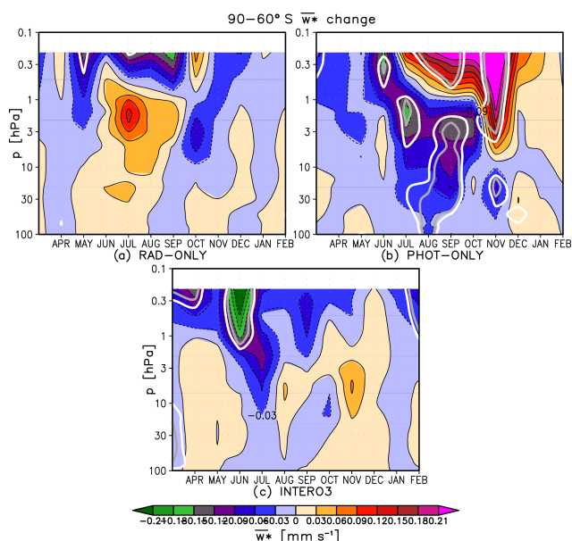
Figure 9. The monthly mean evolution of the polar cap average ( 90\text{--}60^\circ\text{ S} ) change in the vertical component of the transformed Eulerian mean circulation, \bar{w}^* ( \text{mm s}^{-1} ), between SMAX and SMIN for (a) RAD-ONLY, (b) PHOT-ONLY and (c) INTERO3. Positive values indicate anomalous upwelling and vice versa. Thick white and grey lines indicate statistical significance at the 90 % and 95 % confidence level, respectively.
