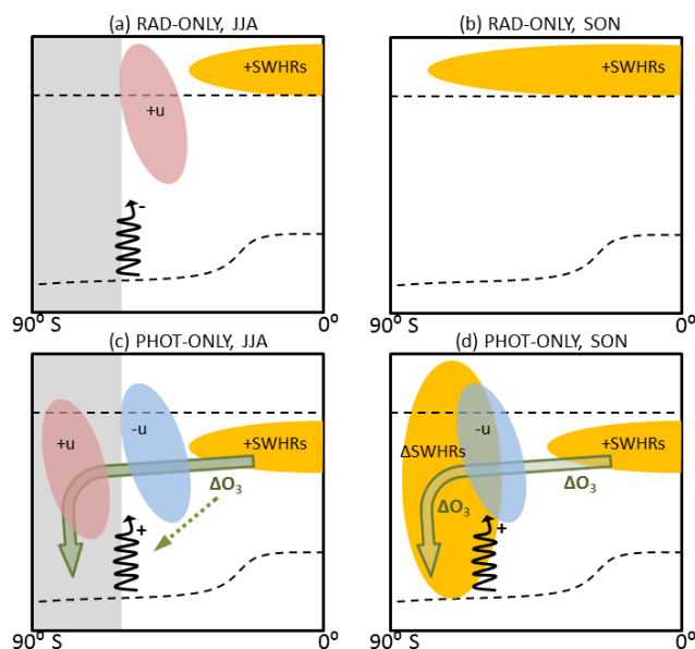
Figure 10. Schematic representation of the proposed mechanism. Yellow ovals represent changes to the SWHRs; red and blue ovals represent strengthening and weakening of zonal mean zonal wind, respectively. The green arrow indicates changes in ozone along the meridional circulation, the wavy black arrows the propagation of planetary waves (increased/decreased as given by the plus/minus signs), and the dotted green line an interaction between ozone and planetary waves. The dashed horizontal lines indicate tropopause and stratopause, and the grey areas in (a, c) indicate the regions covered in polar night.
