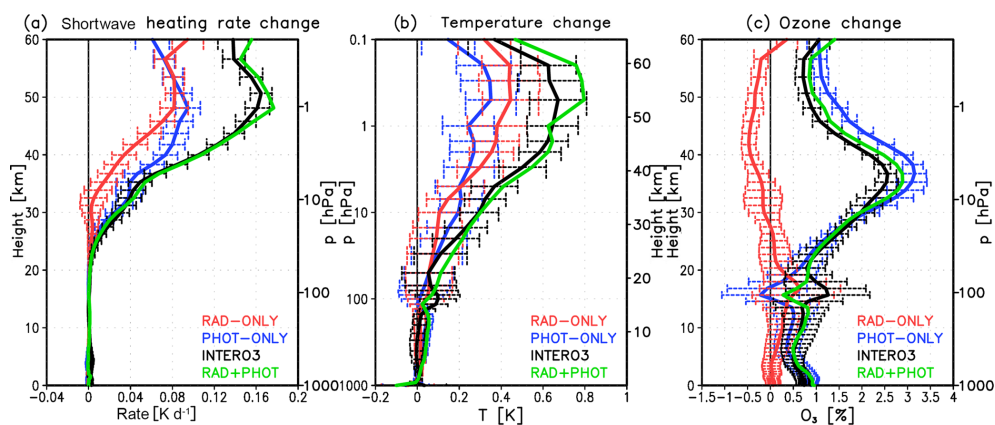
Figure 2. Yearly mean tropical average ( 25^{\circ} N– 25^{\circ} S) change in (a) the shortwave heating rates ( \text{K d}^{-1} ), (b) temperature (K), and (c) ozone (%) between SMAX and SMIN for RAD-ONLY (red), PHOT-ONLY (blue) and INTERO3 (black), together with the associated confidence intervals ( \pm 2 standard errors). The green line indicates the sum of the RAD-ONLY and PHOT-ONLY responses.
