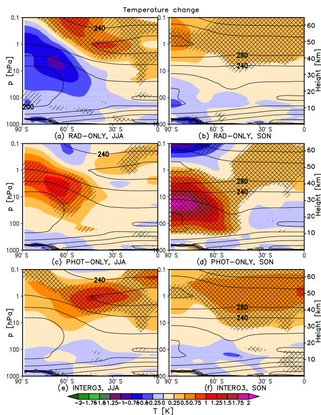
Figure 4. As in Fig. 3 but for the SMAX–SMIN zonal mean temperature changes (K) (shading) and climatological zonal mean temperature in SMIN run (contours). Contours spacing is 20 K (shown for values beginning at 140 K).
