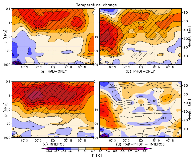
Figure 1. Yearly mean zonal mean temperature change (K) between SMAX and SMIN for (a) RAD-ONLY, (b) PHOT-ONLY and (c) INTERO3. Hatching in (a)–(c) shows regions where the response is statistically significant at the 95 % level (calculated using a two-tailed Student t test). Shown also (d) is the difference (shading) between the sum of the single-forcing responses and INTERO3 (contours, as in c).
