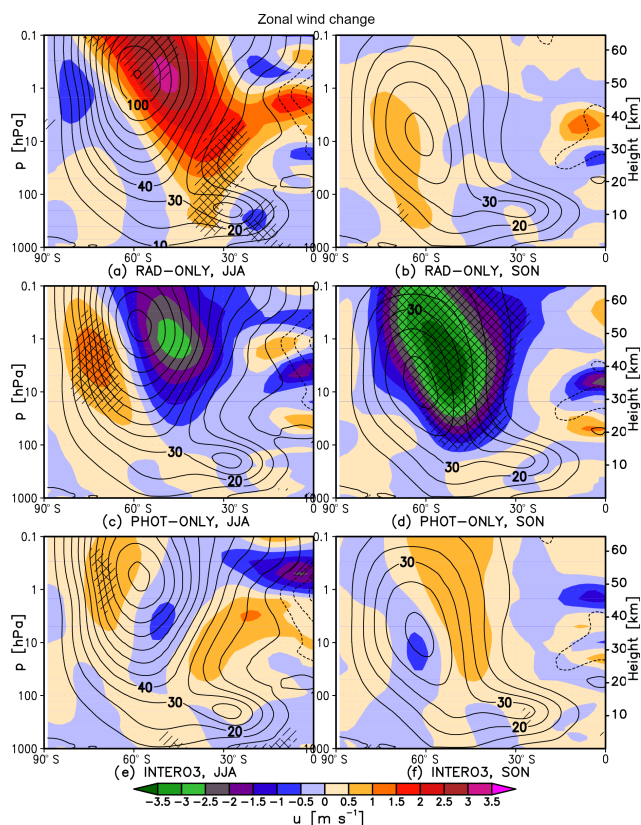
Figure 3. Shading: seasonal mean (left: JJA, and right: SON) SH zonal mean zonal wind change ( \text{m s}^{-1} ) between SMAX and SMIN for (a, b) RAD-ONLY, (c, d) PHOT-ONLY and (e, f) INTERO3. Single and double hatching indicate statistical significance at the 90 % and 95 % confidence level, respectively ( t test). Contours show the corresponding climatological seasonal mean zonal mean zonal wind for the respective SMIN run; contour spacing is 10 \text{ m s}^{-1} .
