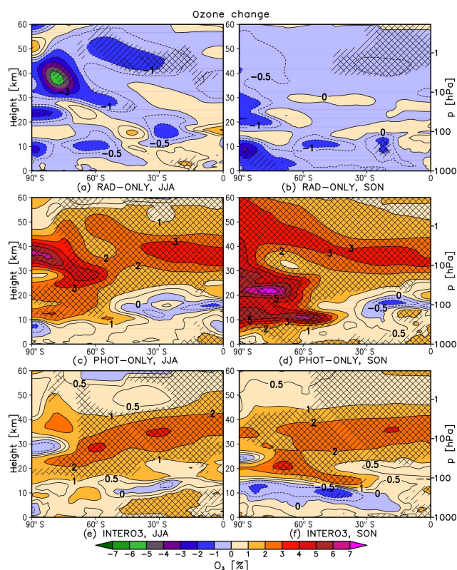
Figure 8. Seasonal mean (left: JJA, right: SON) SH zonal mean changes in ozone mixing ratios (%) between SMAX and SMIN for (a, b) RAD-ONLY, (c, d) PHOT-ONLY and (e, f) INTERO3. Single and double hatching indicate statistical significance at the 90 % and 95 % confidence level, respectively ( t test). Note the additional contours at \pm 0.5 %.
