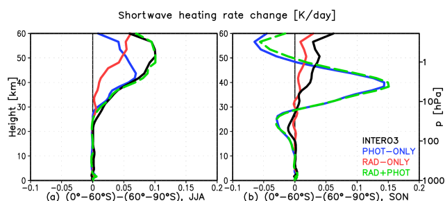
Figure 7. Seasonal mean JJA (a) and SON (b) change in the SWHR gradient ( \text{K d}^{-1} ), as defined in Eq. (4), between SMAX and SMIN for INTERO3 (black), PHOT-ONLY (blue), RAD-ONLY (red), and for the sum of PHOT-ONLY and RAD-ONLY (green).
