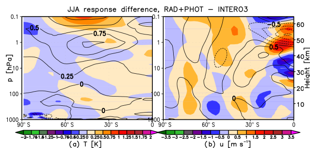
Figure 5. (a) Shading shows the JJA mean difference between the sum of the RAD-ONLY and PHOT-ONLY temperature (K) responses and INTERO3. (b) As in (a) but for the corresponding difference in zonal wind ( \text{m s}^{-1} ) responses. Contours in (a, b) show the responses in INTERO3 for reference.
