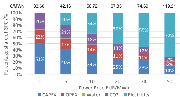
Fig. 4. Percentage share of CAPEX, OPEX, water, CO 2 price and electricity of the GPC of a 10 MW el PtG with perspective cost parameters for 2030 and different power prices.
