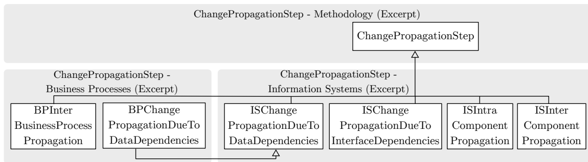
Figure 6.7.: Relationship between the domain-independent ChangePropagationStep and ChangePropagationStep in IS [Sta15], and BP
