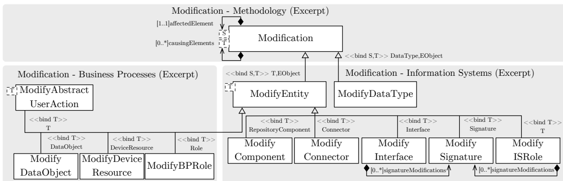
Figure 6.6.: Relationship between the domain-independent Modification and Modification in IS [Sta15], and BP
