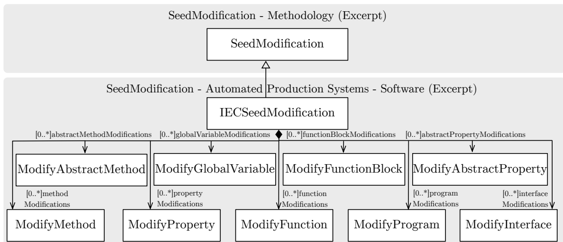
Figure 7.15.: Relationship between the domain-independent SeedModification and the specific SeedModifications in an IEC software [Rät17]
