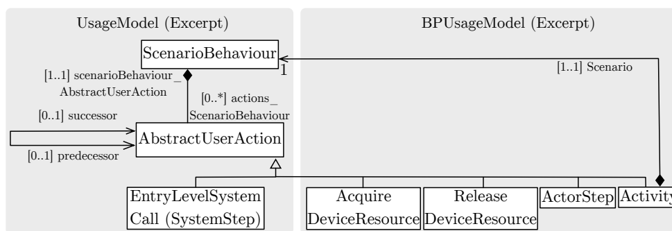
Figure 2.2.: Metamodel of the BP design [Hei14; Hei+17]
