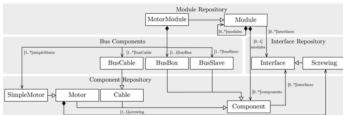
Figure 2.10.: Specific Metamodel of aPS - An excerpt [Koc17; Hei+18]
