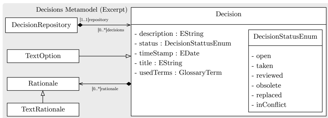
Figure 2.7.: Metamodel of decisions [HS15], adapted from [Küs13; Dur14; DR13]
