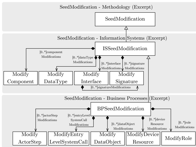
Figure 6.5.: Relationship between the domain-independent SeedModification and SeedModification in IS [Sta15], and BP
