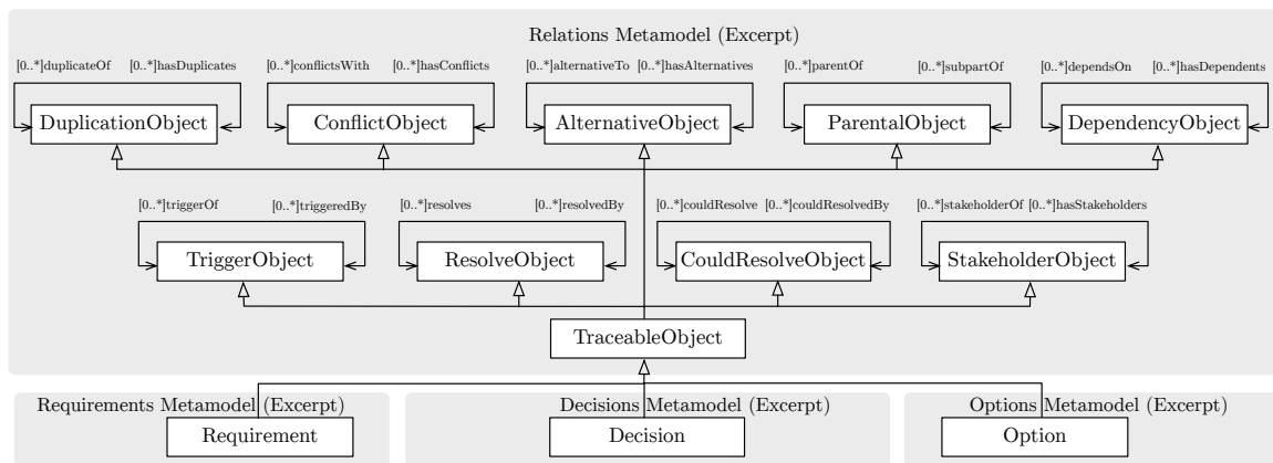
Figure 2.3.: Relationship between requirements, design decisions, and options [HS15], adapted from [Küs13; Dur14; DR13]
