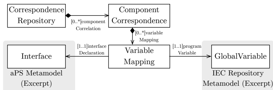
Figure 7.2.: Correspondence model illustrating the relationship between communication interfaces of a PLC and global variables in the control software [Rät18; Koc17; Hei+18]
