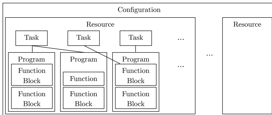
Figure 2.8.: Simplified structure of an IEC program, adapted from the IEC software model [IEC13]
