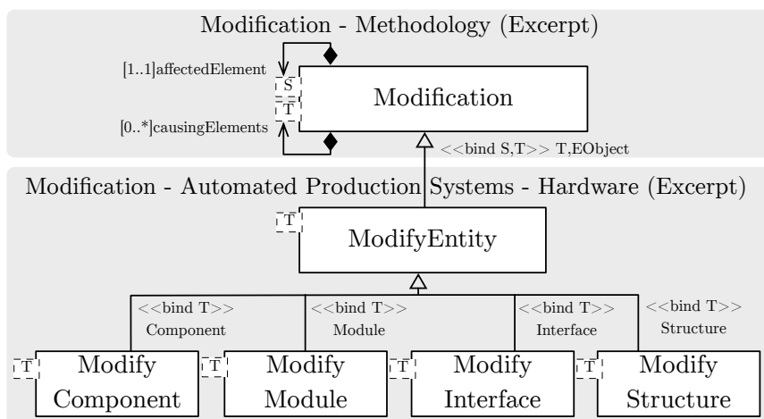
Figure 7.4.: Relationship between the domain-independent Modification and Modification in mechanical and electrical/electronic elements
