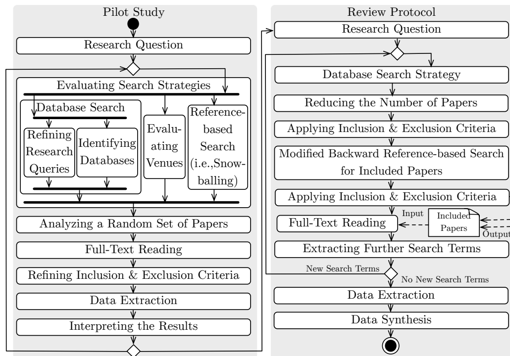
Figure 10.1.: Overview of the review process involving the pilot study and the review protocol as an activity diagram [Kap+18a, p. 2]
