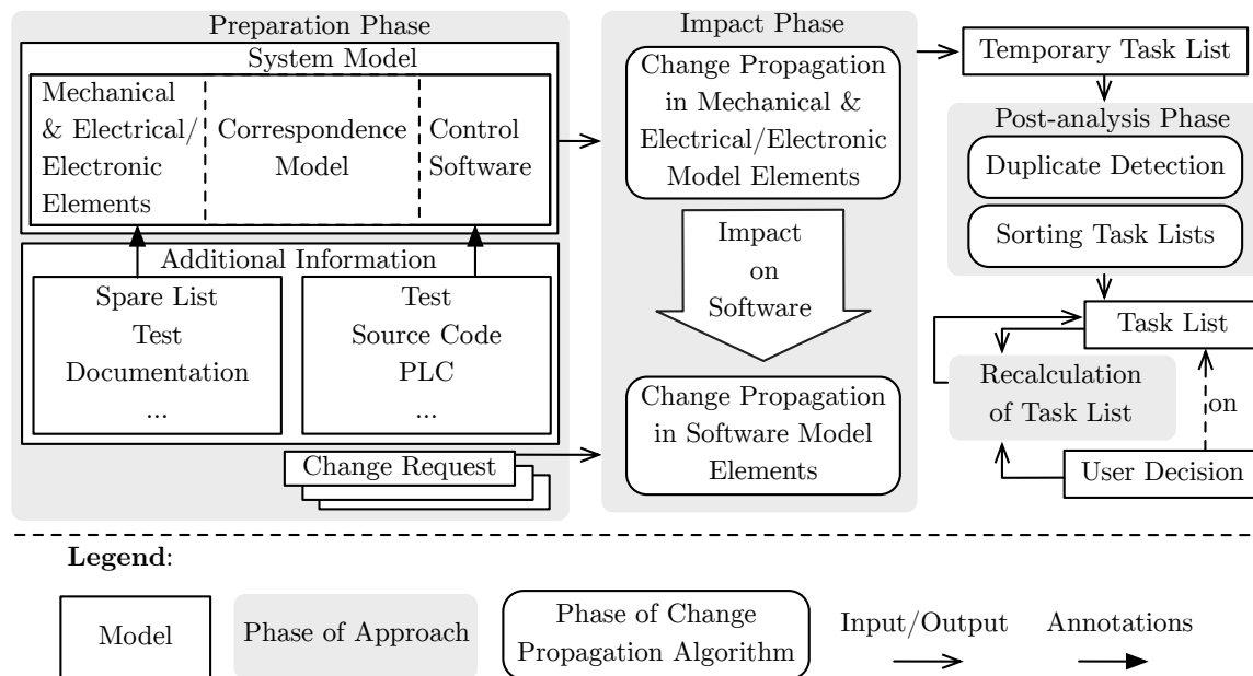
Figure 7.1.: Overview of the KAMP4aPS approach
