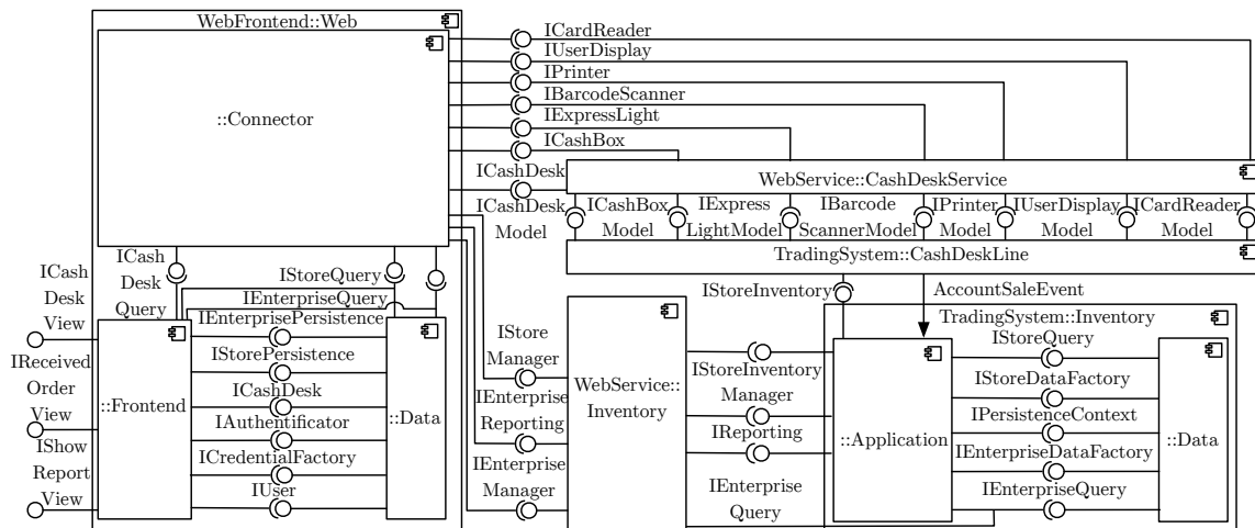
Figure 11.2.: Component diagram of CoCoME [HRR16; Ros+17a]
