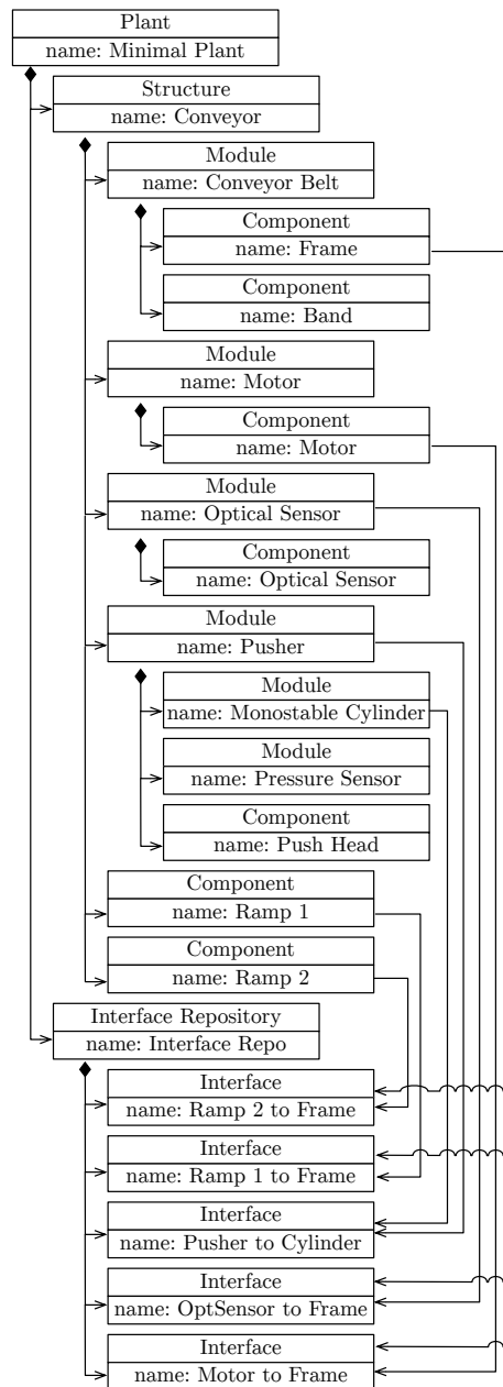
Figure 4.3.: Overview of the hardware of the Minimal Plant example as a reduced variant of the xPPU [Vog+14a]
