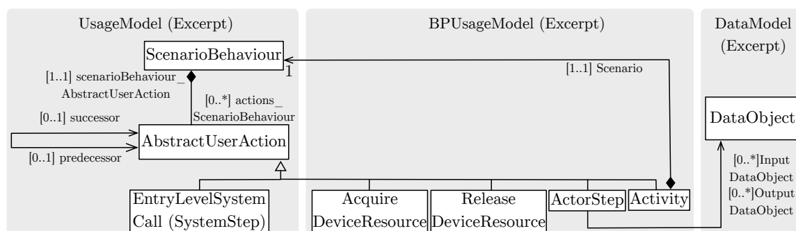
Figure 6.4.: Relationship between PCM UsageModel [BKR09], BPUUsageModel [Hei+17], and DataModel [Ros+17a]
