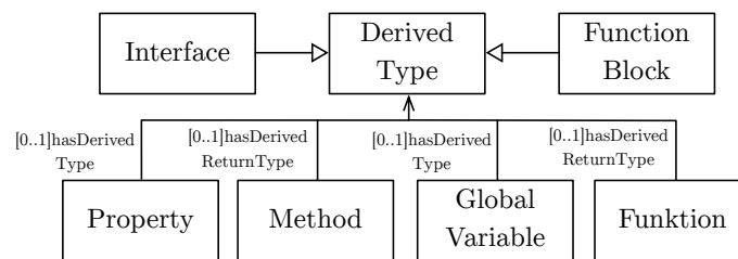
Figure 7.13.: Metamodel of IECRepository involving DerivedType - An excerpt [Rät17]
