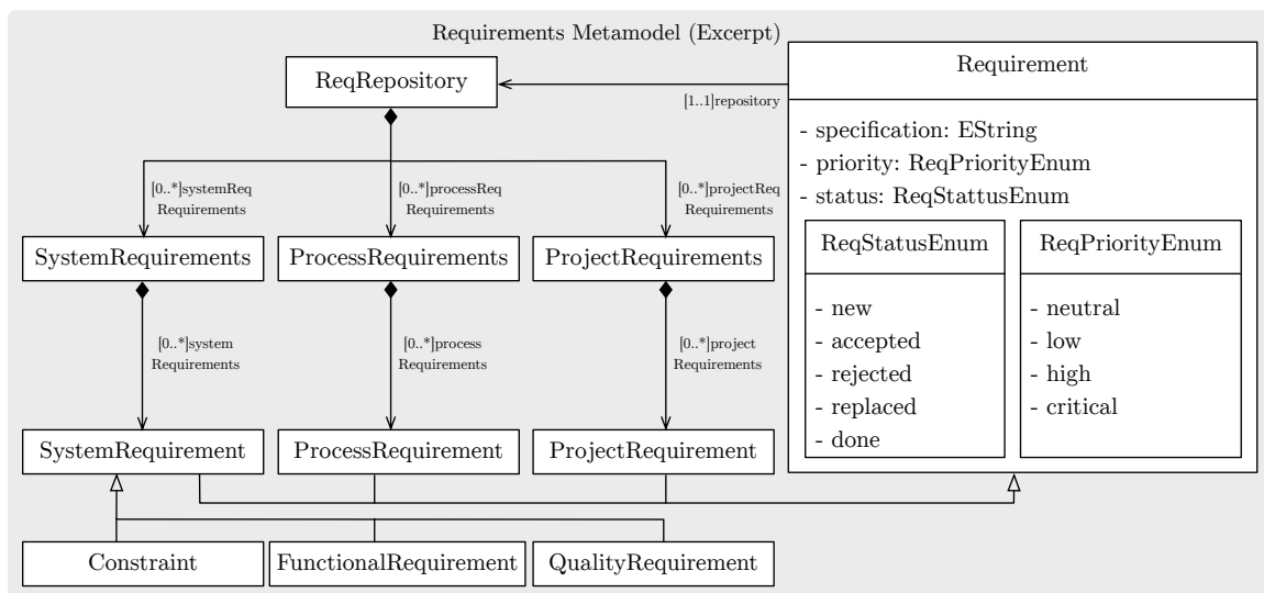
Figure 2.4.: Metamodel of requirements [HS15], adapted from [Küs13; Dur14; DR13]
