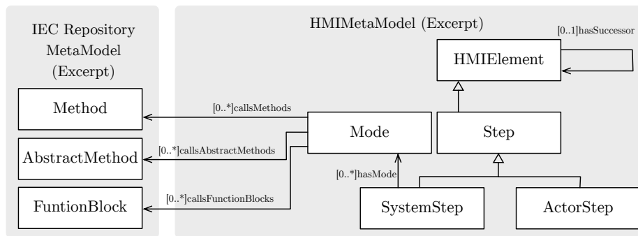
Figure 7.14.: Metamodel of the HMI involving ActorStep and SystemStep - An Excerpt [Rät18]
