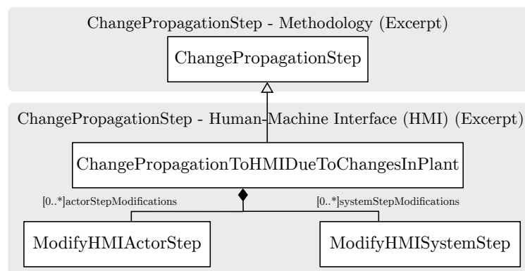
Figure 7.20.: Relationship between the domain-independent ChangePropagationStep and the specific ChangePropagationSteps in an HMI [Rät18]
