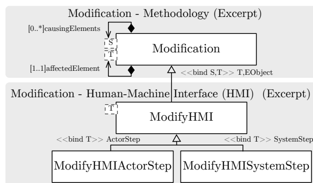
Figure 7.18.: Relationship between the domain-independent Modification and the specific Modifications in an HMI [Rät18]
