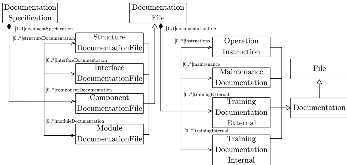
Figure 7.8.: Documentation specifications for mechanical, electrical/electronic elements [Koc17] based on [Sta15]
