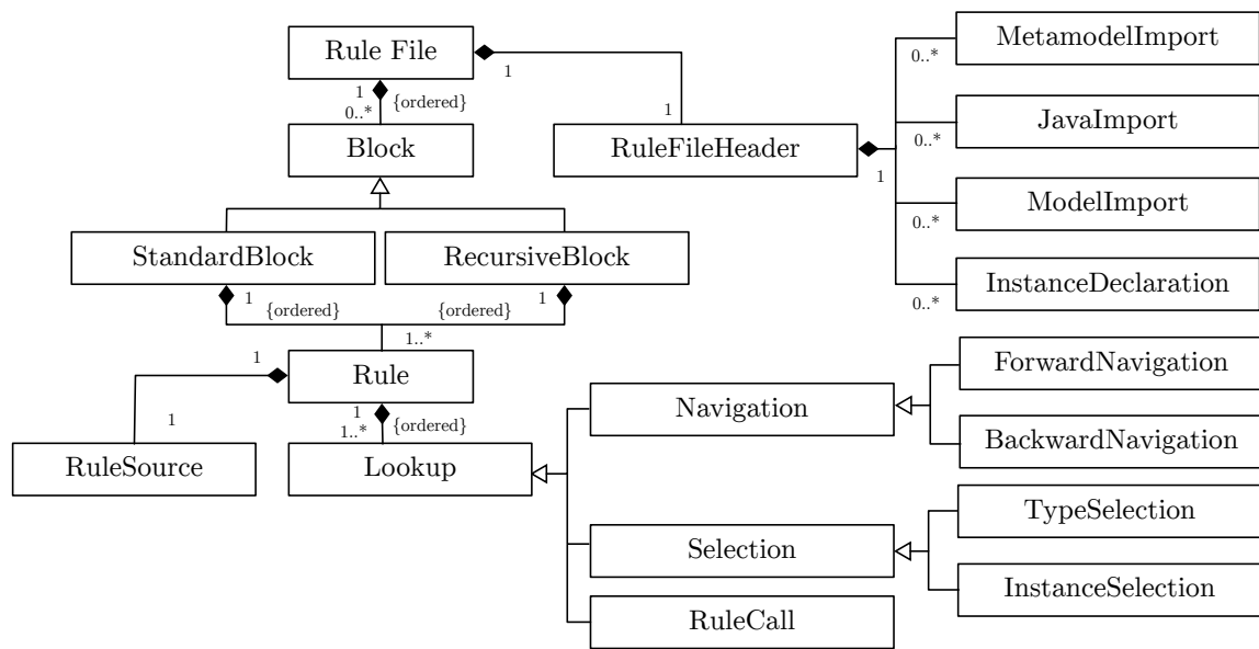
Figure 9.4.: A reduced and simplified illustration of the relevant elements of CPRL as class diagram, adapted from [Bus+18b; Löp18]
