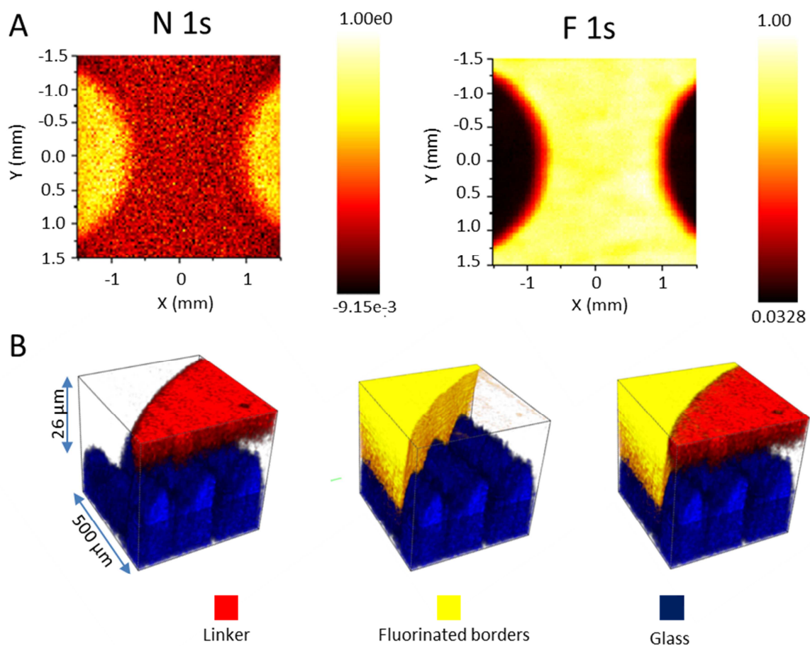
Fig. 3. Experiments proving the confinement of liquids inside hydrophilic spots. A) XPS image of the area between spots depicting the abundance of nitrogen inside the spots (left image, assigned to the amide and nitro group, N 1s, 400.2 and 406.0 eV respectively) and fluorine outside the spots (right image, assigned to the fluorine, F 1s, 689.0 eV). B) 3D rendering of ToF-SIMS depth profiles; linker, characterized by \text{NO}_2^- (red), fluorinated borders, characterized by F- (yellow) and glass substrate ( \text{SiO}_2^- , \text{SiO}_3^- , and \text{SiO}_3\text{H}^- ) (blue). X-Y-Dimensions are 500x500 μm.
