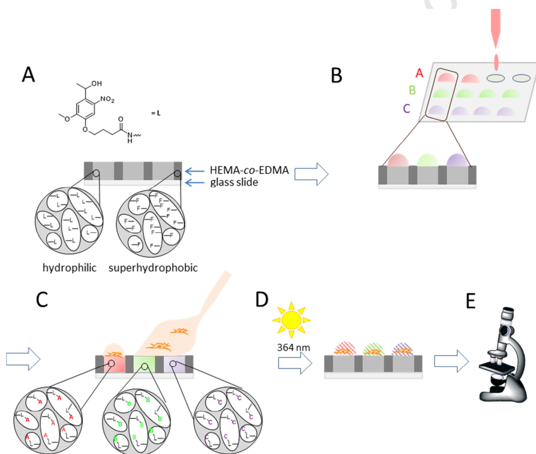
Fig. 1. General workflow of solid-phase synthesis using ChemBIOS platform with photocleavable linkers. A) Superhydrophobic-hydrophilic microarray with hydrophilic spots functionalized with photolinkers L . B) Synthesis of a combinatorial library of small molecules; C) Seeding of cells to form an array of aqueous droplets. D) The screening experiment can be started on demand by irradiating all or selected droplets with 364 nm UV light (1-15 min) E) Read-out step.
