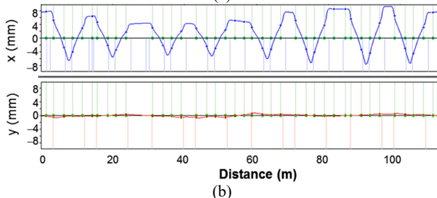
Figure 5: Negative- \alpha operation: Oscillations of beam orbit in the ring. Similar results were obtained for positive low- \alpha optics at injection: (a) measured data, blue/red curves – horizontal/vertical position; (b) simulations for beam trajectory with energy offset and random misalignment errors \sigma_x=30 \mu , \sigma_y=10 \mu , energy of injected beam is less than reference orbit energy at \delta = -0.35\% .
