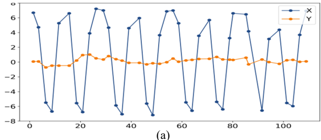
Figure 3: Trajectory of injected beam at low- \alpha settings of ring quads before correction of K1, K2 and K3 kickers.
