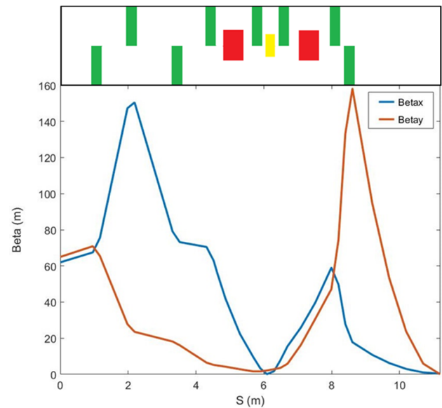
Figure 7: Evolution of beta functions along the beam line from the exit of the Linac up to the entrance of the TGU.
