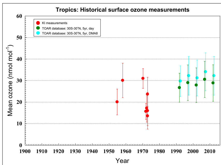
Figure 5: Historical measurements of surface ozone in the tropics ( 30^{\circ}\text{S} – 30^{\circ}\text{N} ; see Table 6 for details). Error bars represent standard deviations of the measurement averages (atmospheric variability), not measurement uncertainty. Five-year averages (daytime mean) of modern UV measurements at sites below 2000 m, classified as “rural”, in the TOAR 5 \times 5 degree gridded average product are also shown, both daytime averages (day) and daily 8-hour maxima (DMA8) (Schultz et al., 2017). DOI: https://doi.org/10.1525/elementa.376.f5
