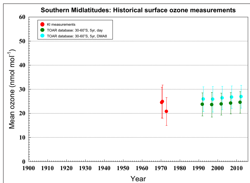
Figure 6: Historical measurements of surface ozone in the Southern Temperate region ( 30^{\circ}\text{S} – 60^{\circ}\text{S} ; see Table 6 for details). Error bars represent standard deviations of the measurement averages (atmospheric variability), not uncertainty of the measurement. Five-year averages (daytime mean) of modern UV measurements at sites below 2000 m, classified as “rural”, in the TOAR 5 \times 5 degree gridded average product are also shown, for both daytime averages (day) and daily 8-hour maxima (DMA8) (Schultz et al., 2017). DOI: https://doi.org/10.1525/elementa.376.f6
