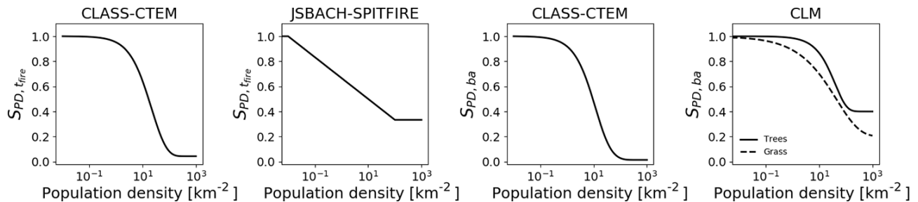
Figure 8. Suppression effects of population density on fire duration ( SPD, t_{fire} ) for CLASS-CTEM and JSBACH SPITFIRE and suppression effects on fire size ( SPD, ba ) for CLASS-CTEM and CLM. All models are scaled to the value range (0,1).
